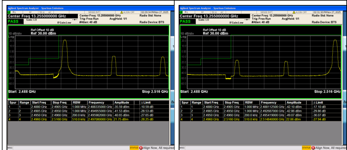
Band41_20MHz_16QAM_39750_1RB#0
