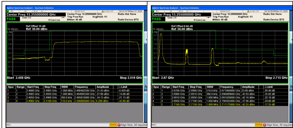
Band41_20MHz_QPSK_39750_100RB#0
