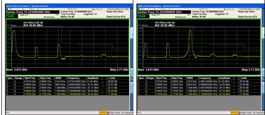
Band41_15MHz_16QAM_41515_1RB#0
