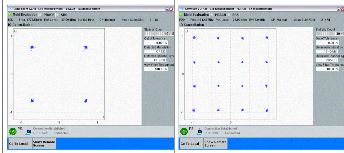
Band66-5MHz-QPSK-132647-25RB#0-PASS
