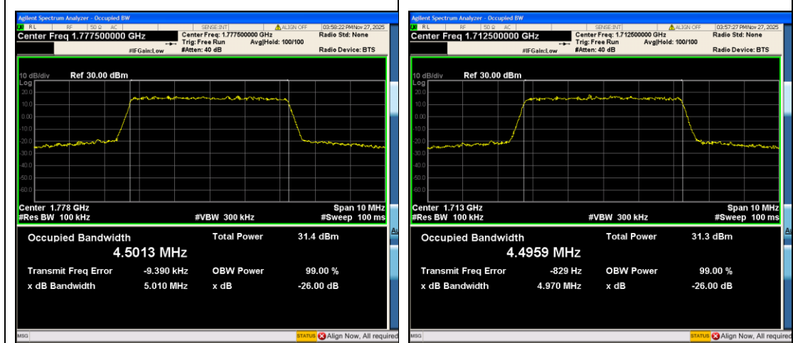
Band66-5MHz-QPSK-132647-25RB#0-PASS
