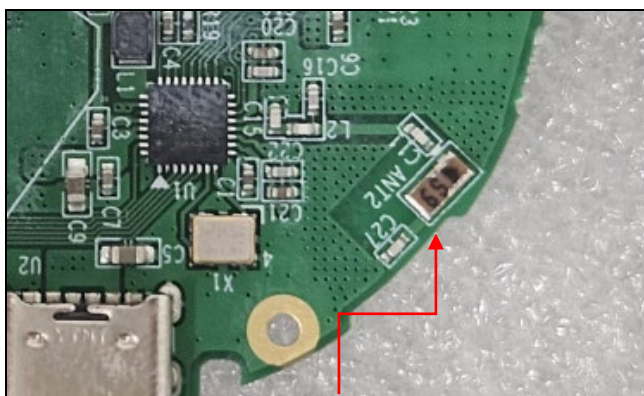
Chip Antenna
