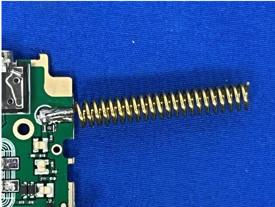
Spring Antenna
