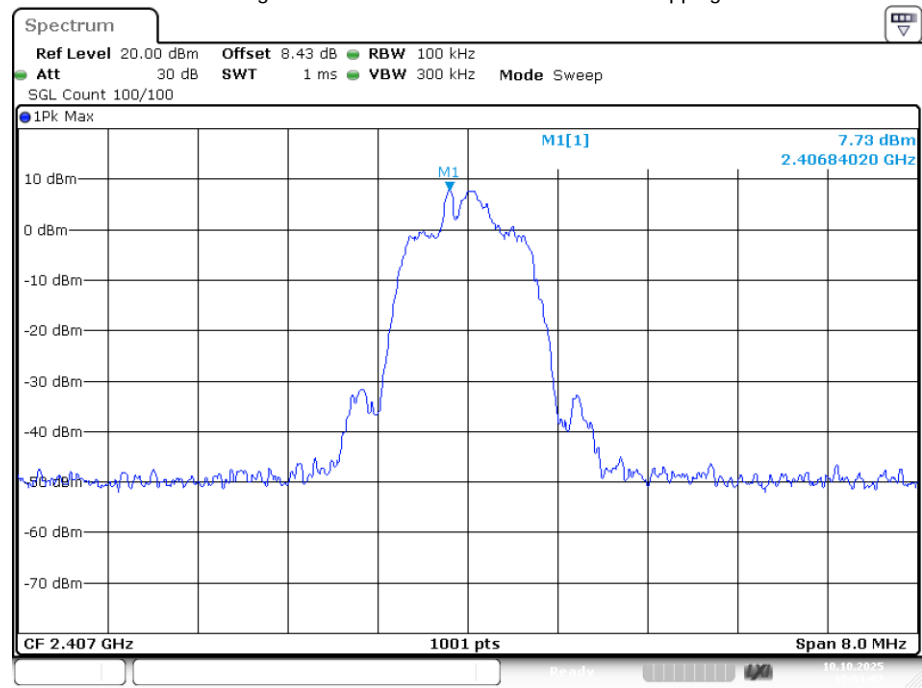
Band Edge NVNT 2.4G Mode 2407MHz Ant1 No-Hopping Ref
