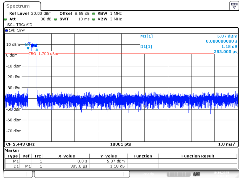
Dwell NVNT 2.4G Mode 2443MHz Ant1 One Burst
