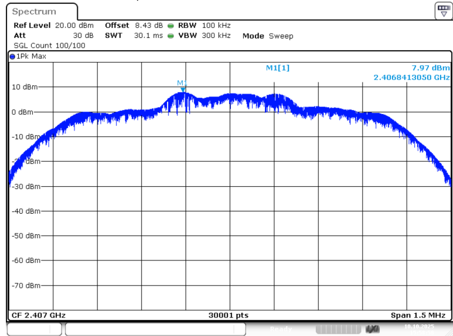
Tx. Spurious NVNT 2.4G Mode 2407MHz Ant1 Ref
