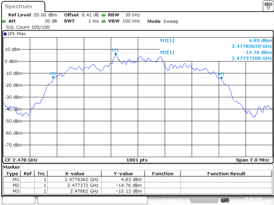
-20dB Bandwidth NVNT 2.4G Mode 2478MHz Ant1
