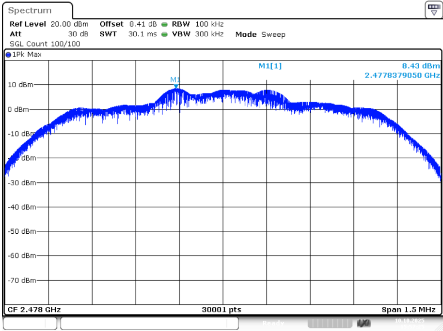
Tx. Spurious NVNT 2.4G Mode 2478MHz Ant1 Ref
