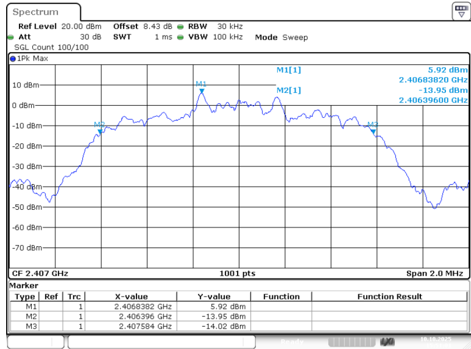
-20dB Bandwidth NVNT 2.4G Mode 2407MHz Ant1
