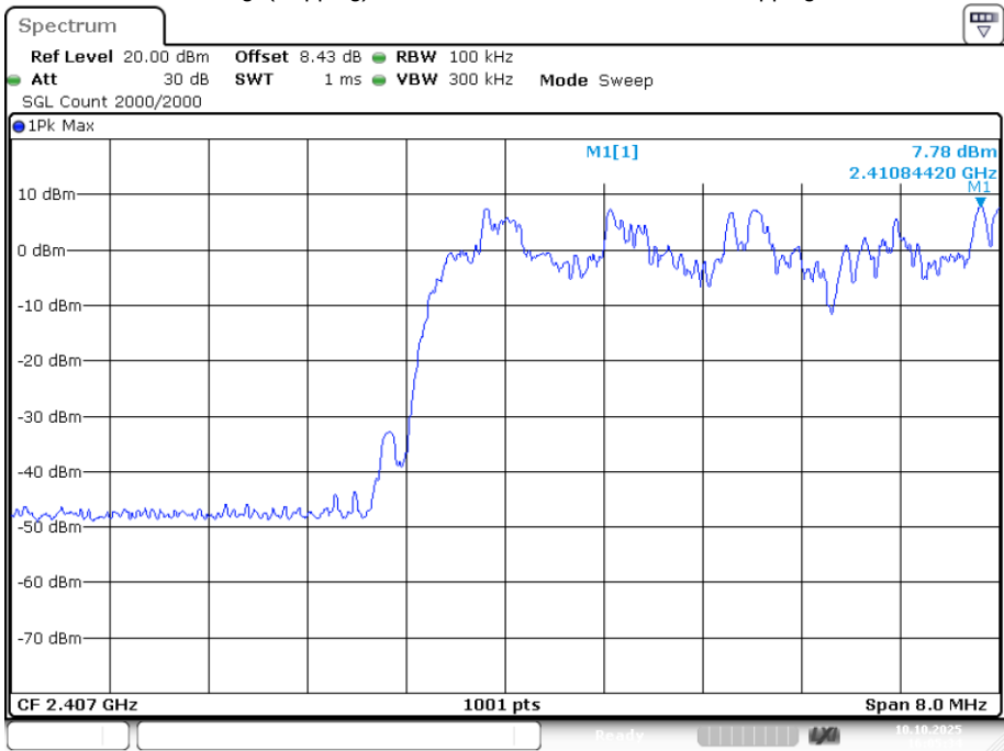
Band Edge(Hopping) NVNT 2.4G Mode 2407MHz Ant1 Hopping Ref
