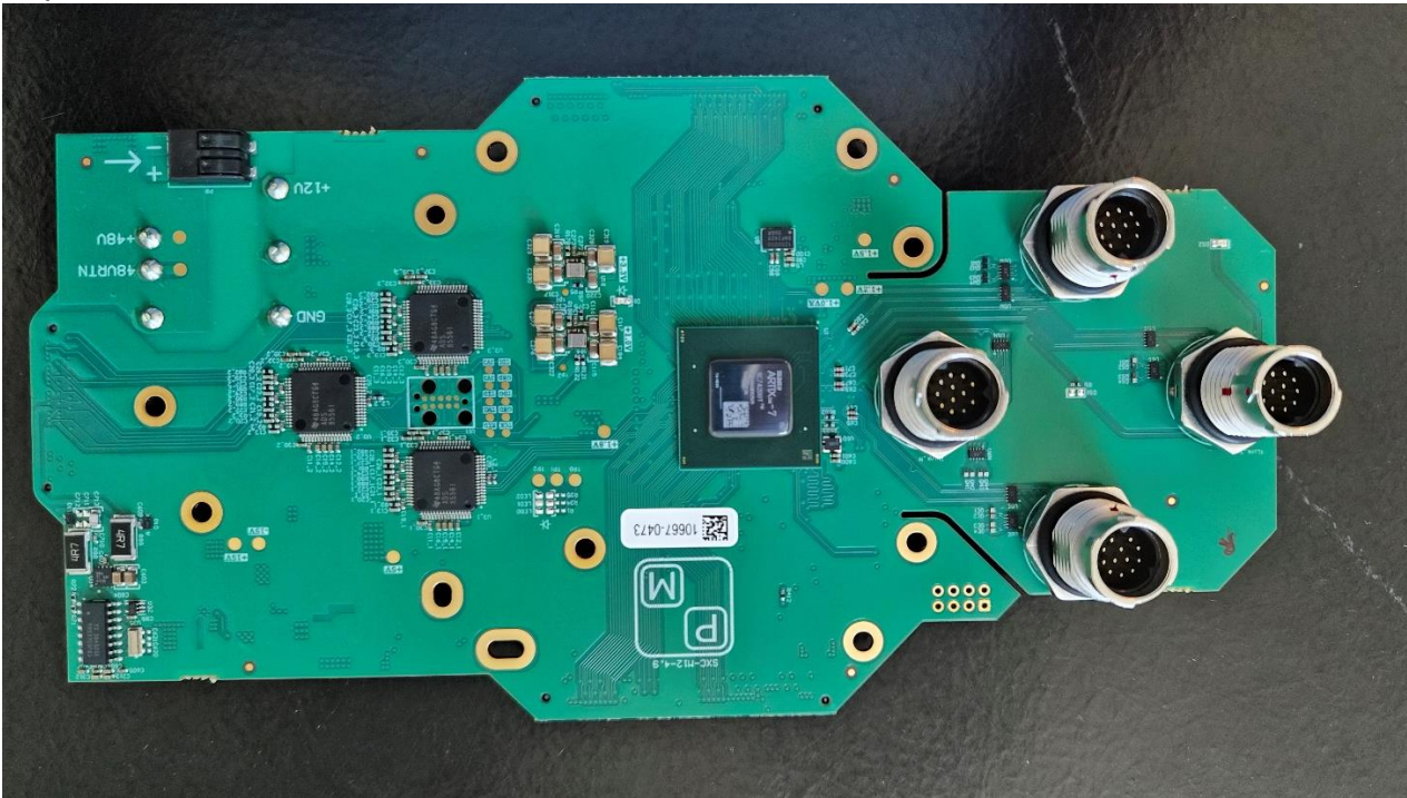
Bottom of controller
