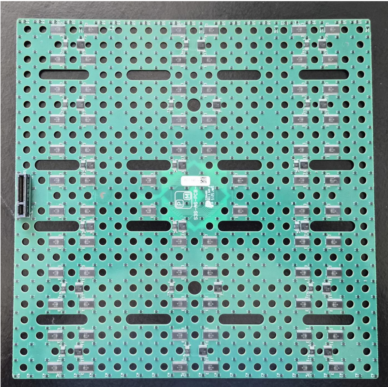
Bottom of sensor board (antenna shown in center)
