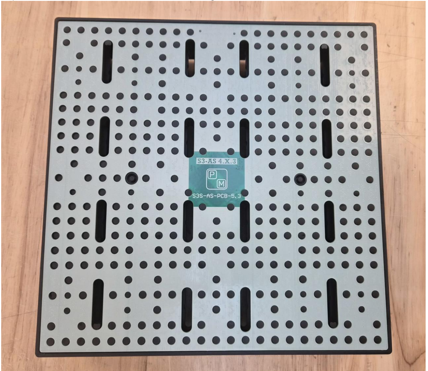
Top down view of sensor board installed in housing
