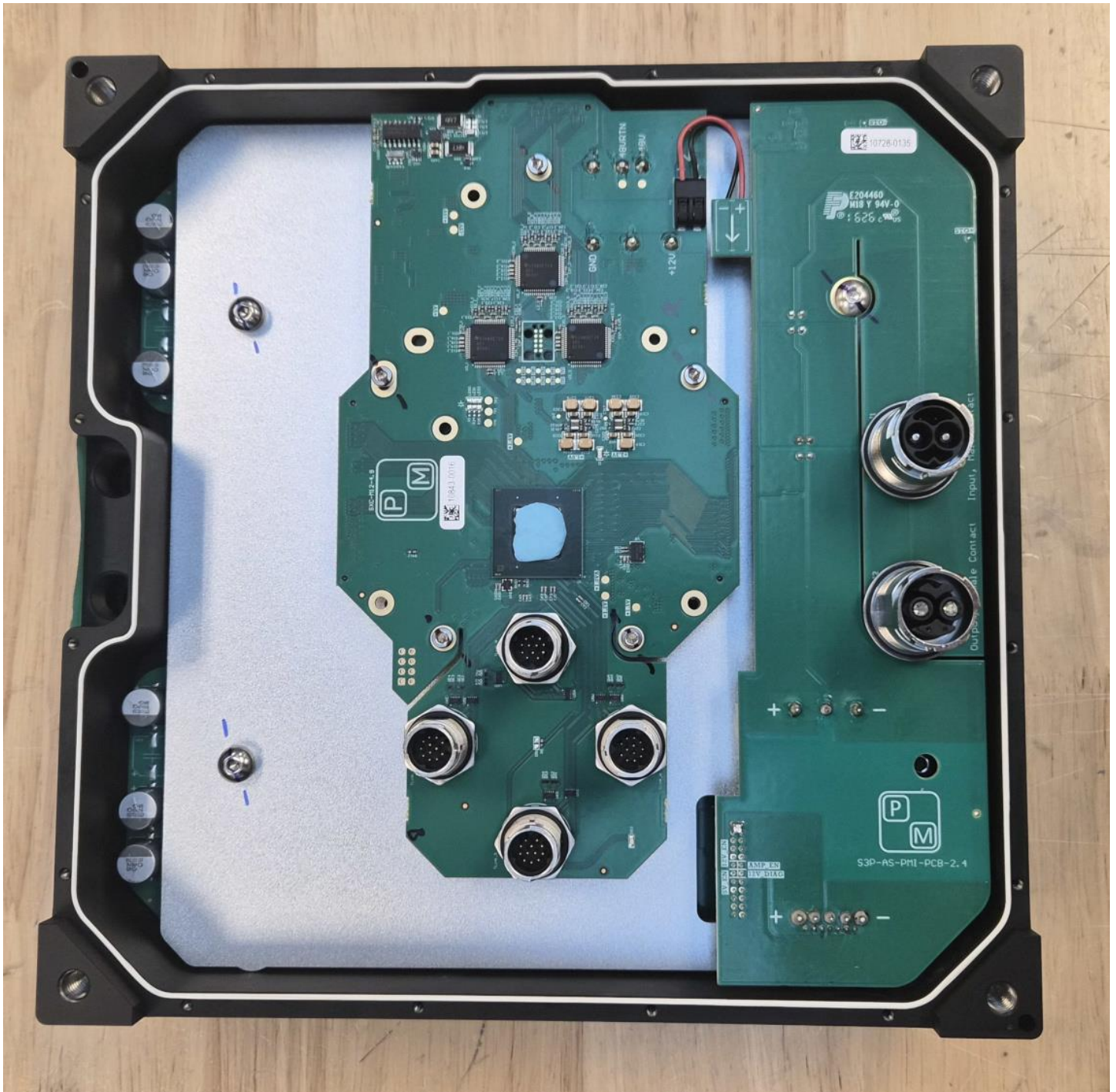
Top down view of controller installed in housing
