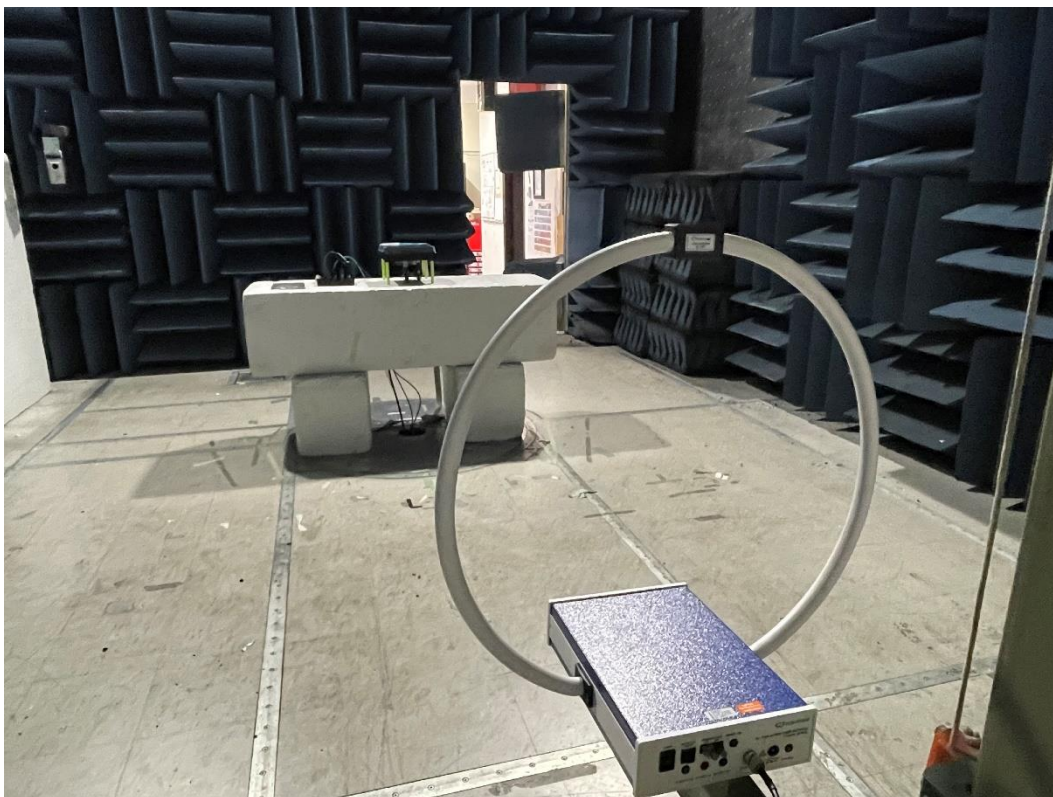
Test setup of radiated emissions below 30 MHz
