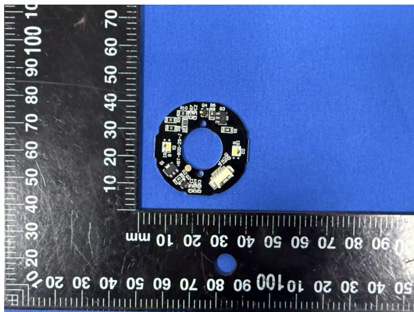
EUT PHOTO 4-PCB view
