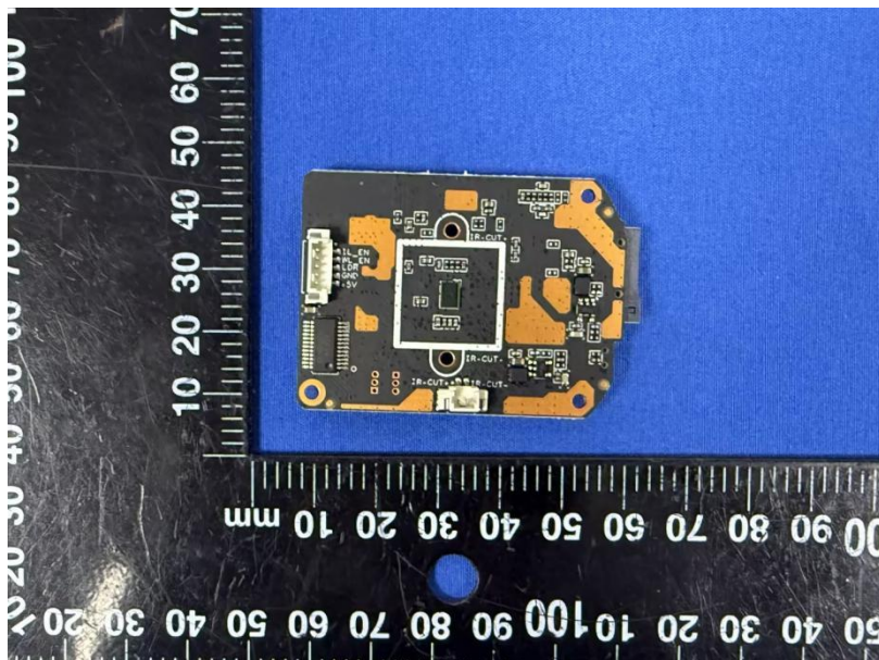
EUT PHOTO 2-PCB view
