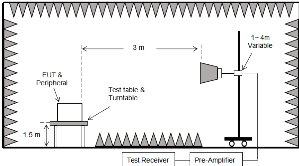
Figure 3. Above 1 GHz
