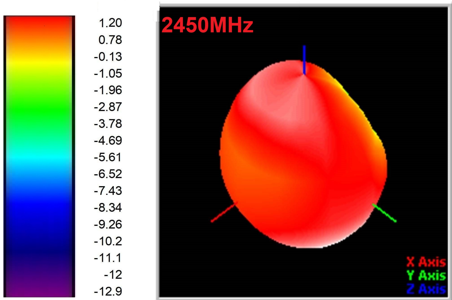
3D radiation pattern diagram
