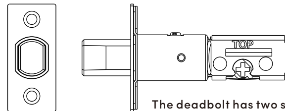
General door's installation diagram
