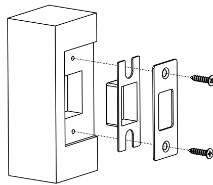
General door's installation diagram
