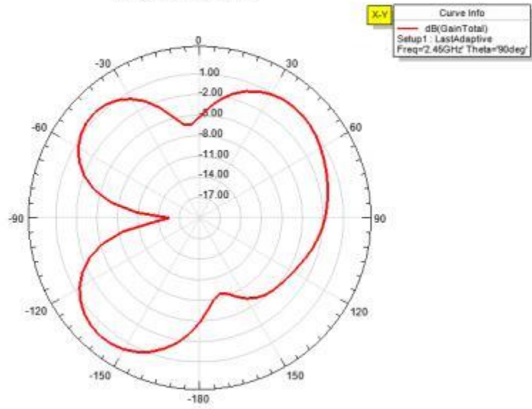
Radiation Pattern 2
