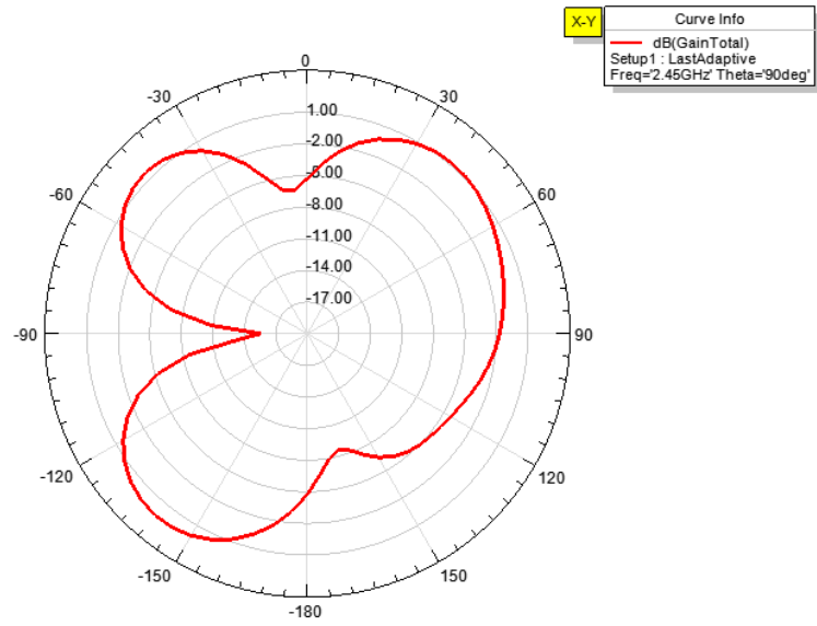
Radiation Pattern 2
