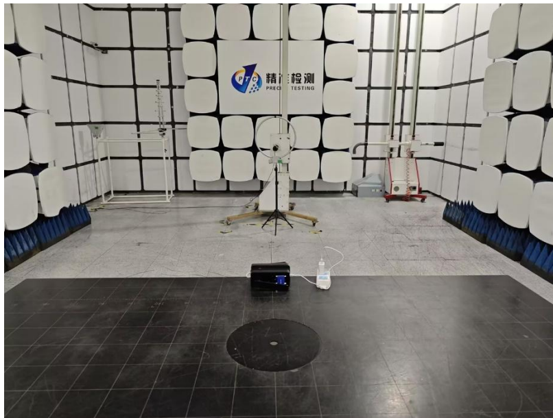
RADIATED EMISSION TEST Test Frequency From 9kHz to 30MHz
