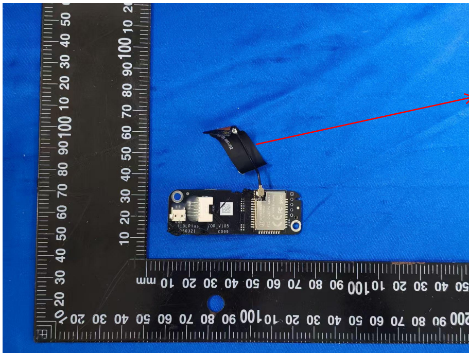
WiFi Antenna
