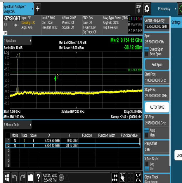
BLE_1M-Ant1-2440-1000~26500-PASS
