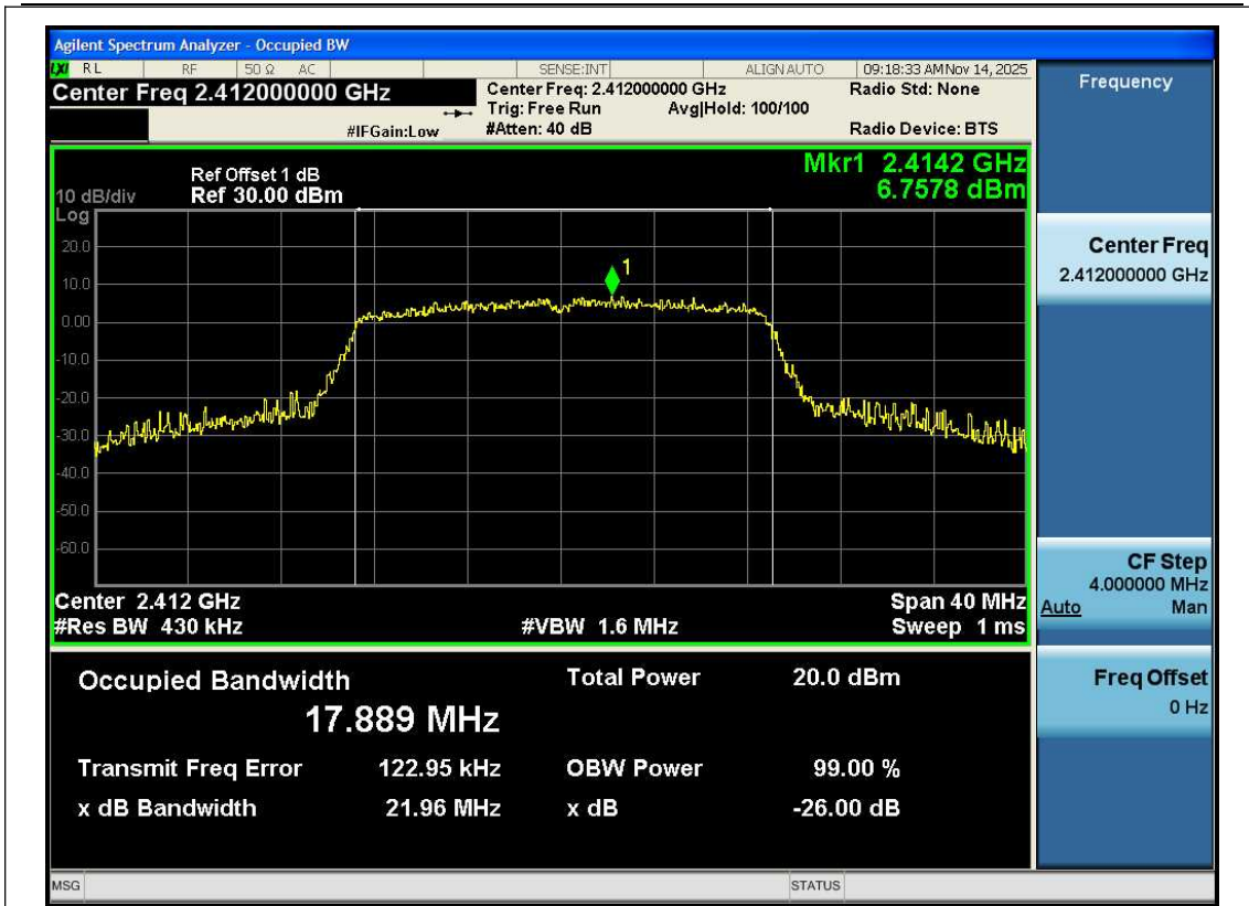
11N20SISO-Ant1-2412
