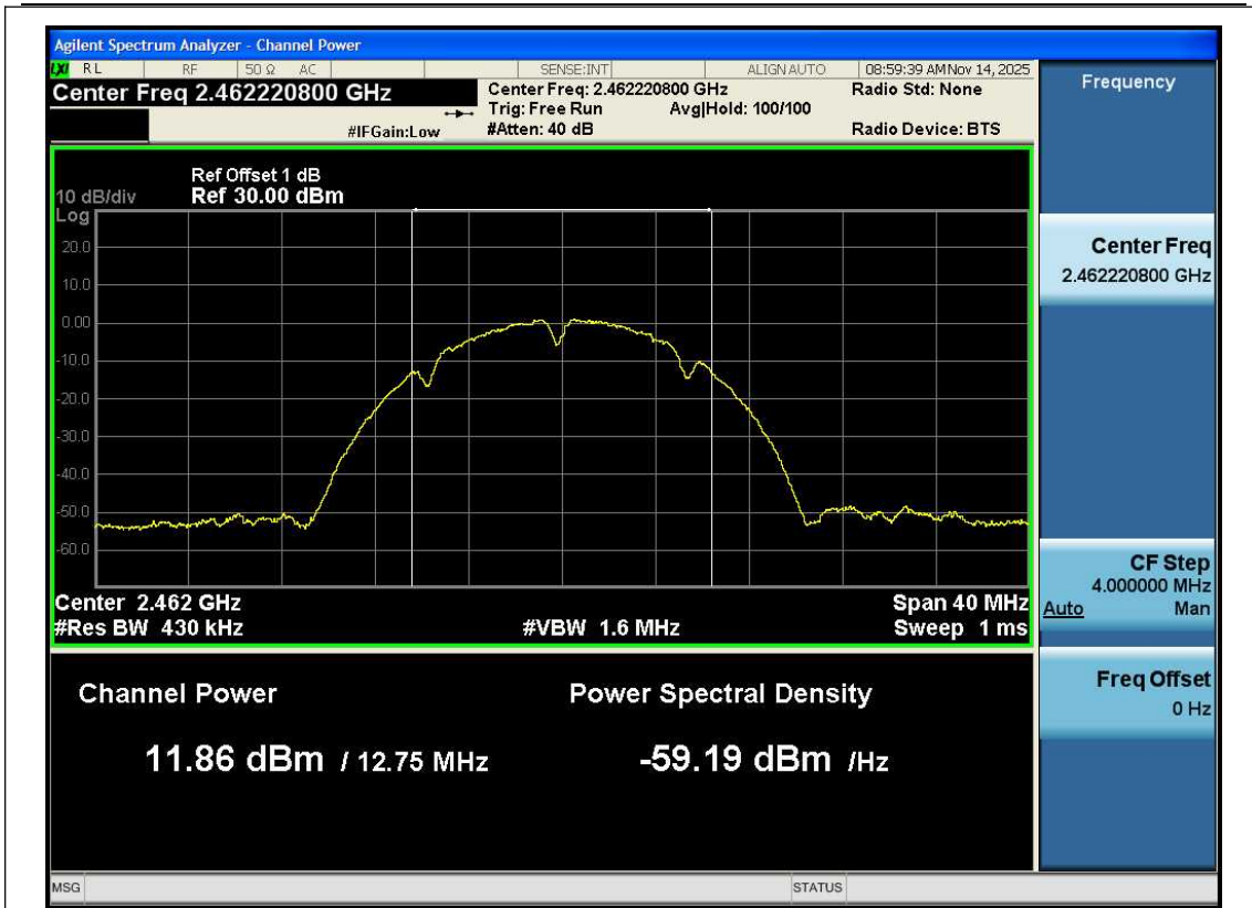
11B-Ant1-2462-PASS
