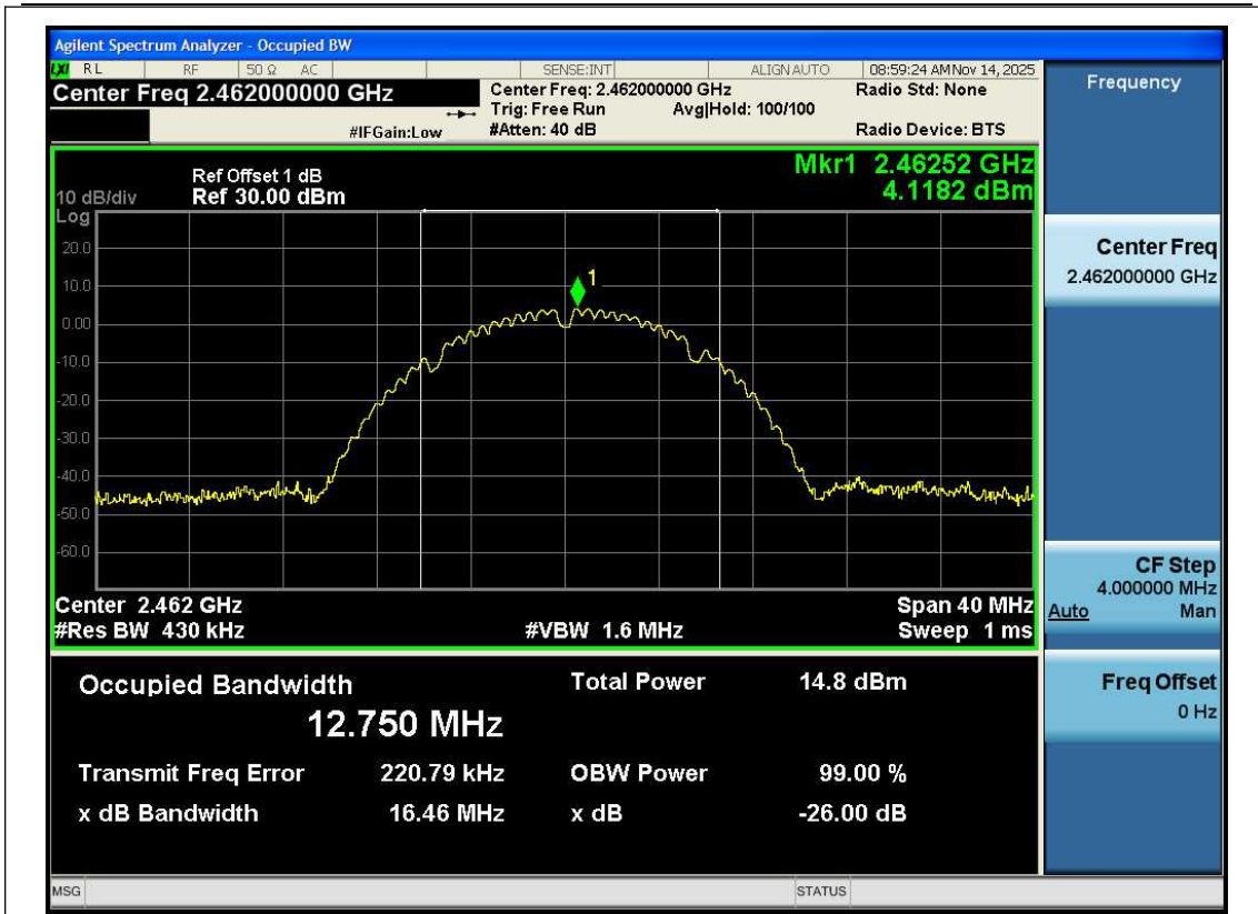
11B-Ant1-2462
