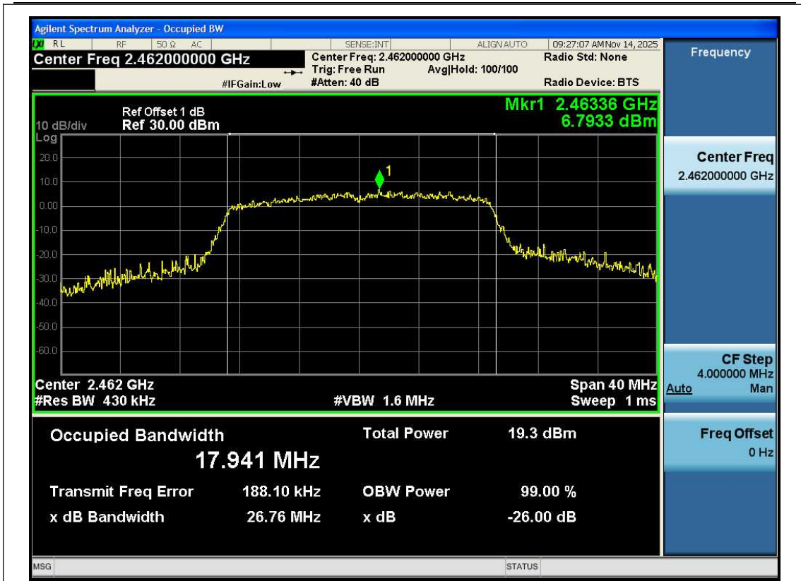
11N20SISO-Ant1-2462
