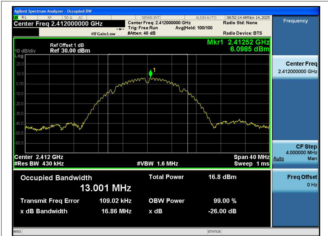
11B-Ant1-2412
