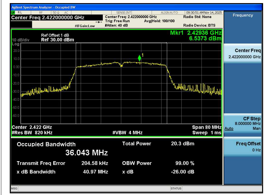
11N40SISO-Ant1-2422
