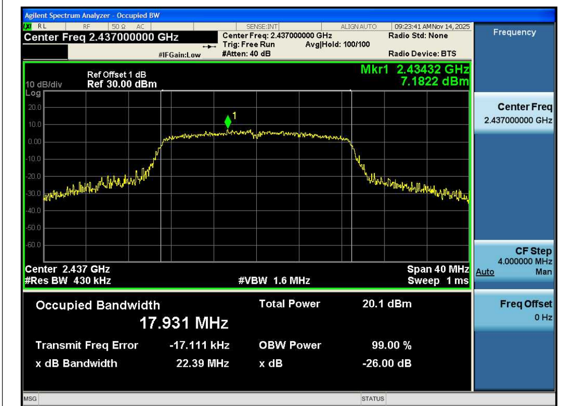
11N20SISO-Ant1-2437
