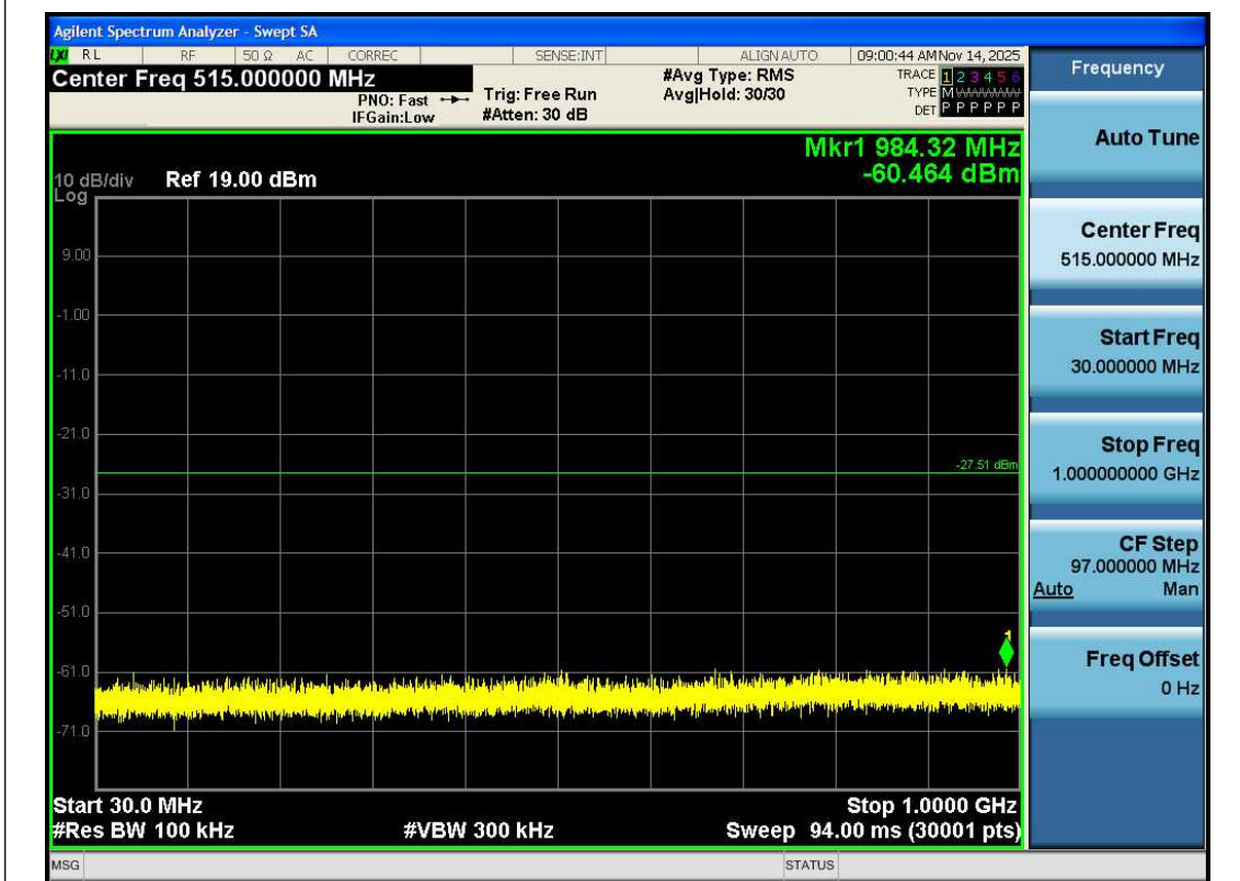
11B-Ant1-2462-30~1000-PASS
