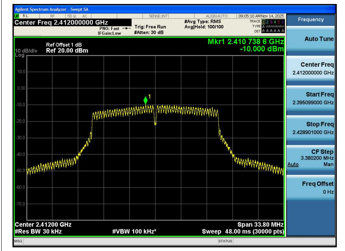
11G-Ant1-2412-PASS
