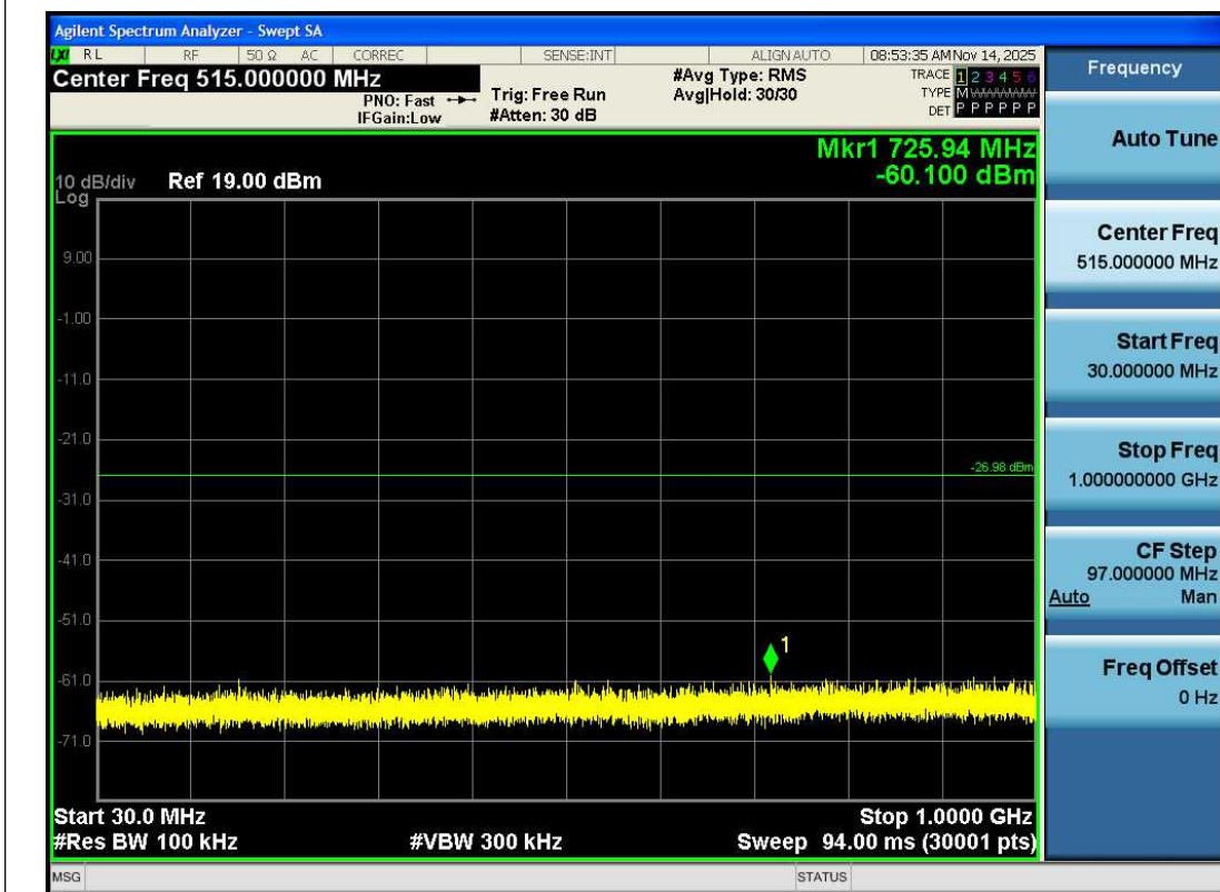
11B-Ant1-2412-30~1000-PASS
