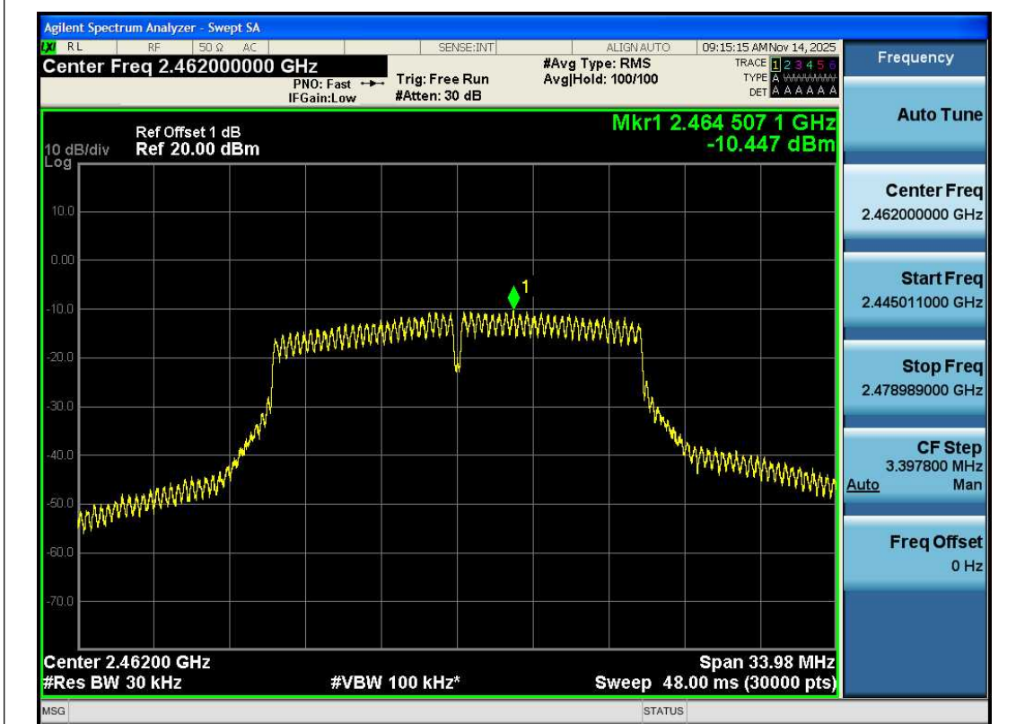
11G-Ant1-2462-PASS
