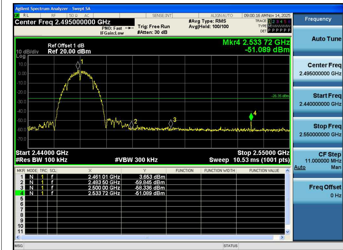
11B-Ant1-2462-PASS
