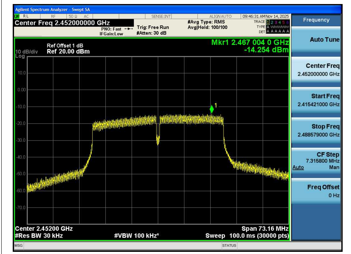
11N40SISO-Ant1-2452-PASS
