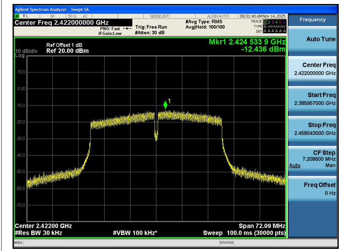
11N40SISO-Ant1-2422-PASS
