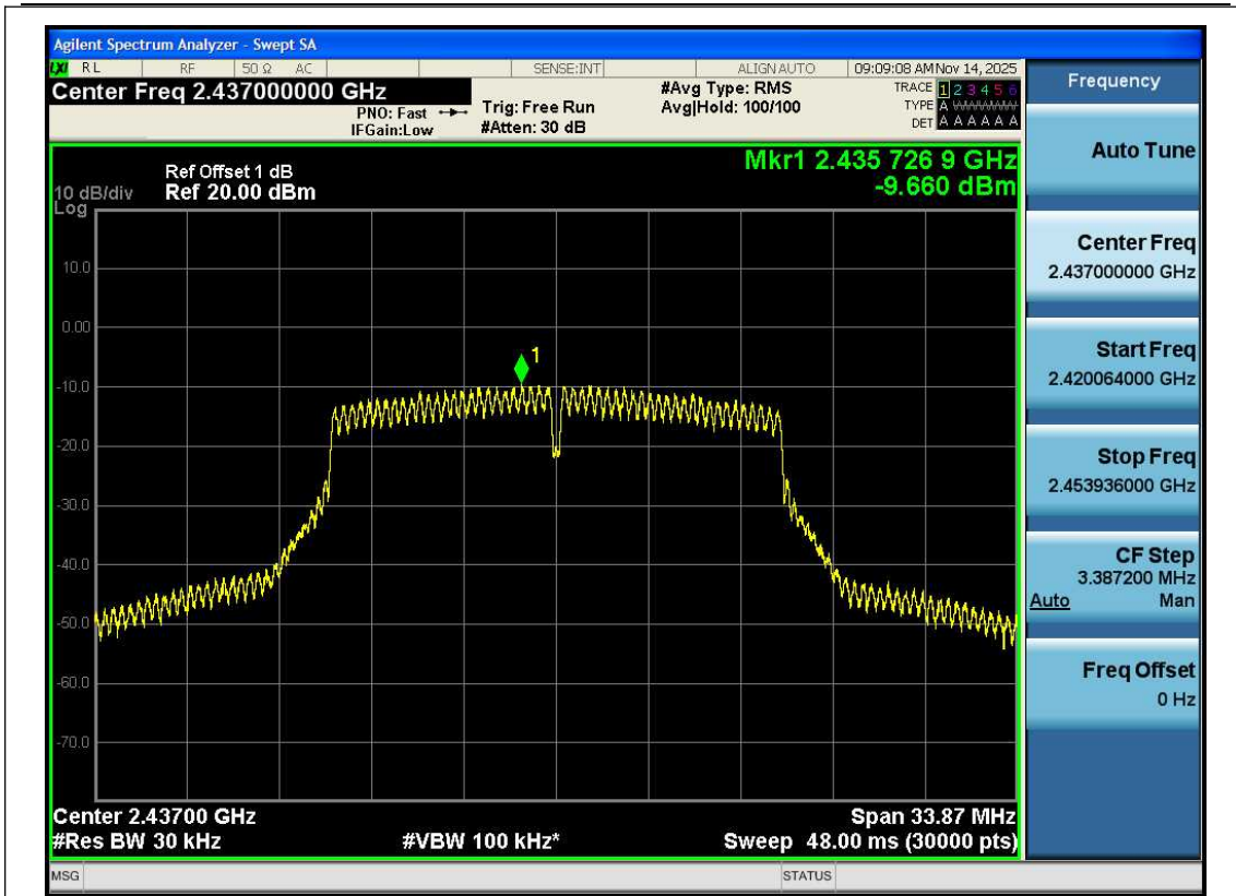
11G-Ant1-2437-PASS
