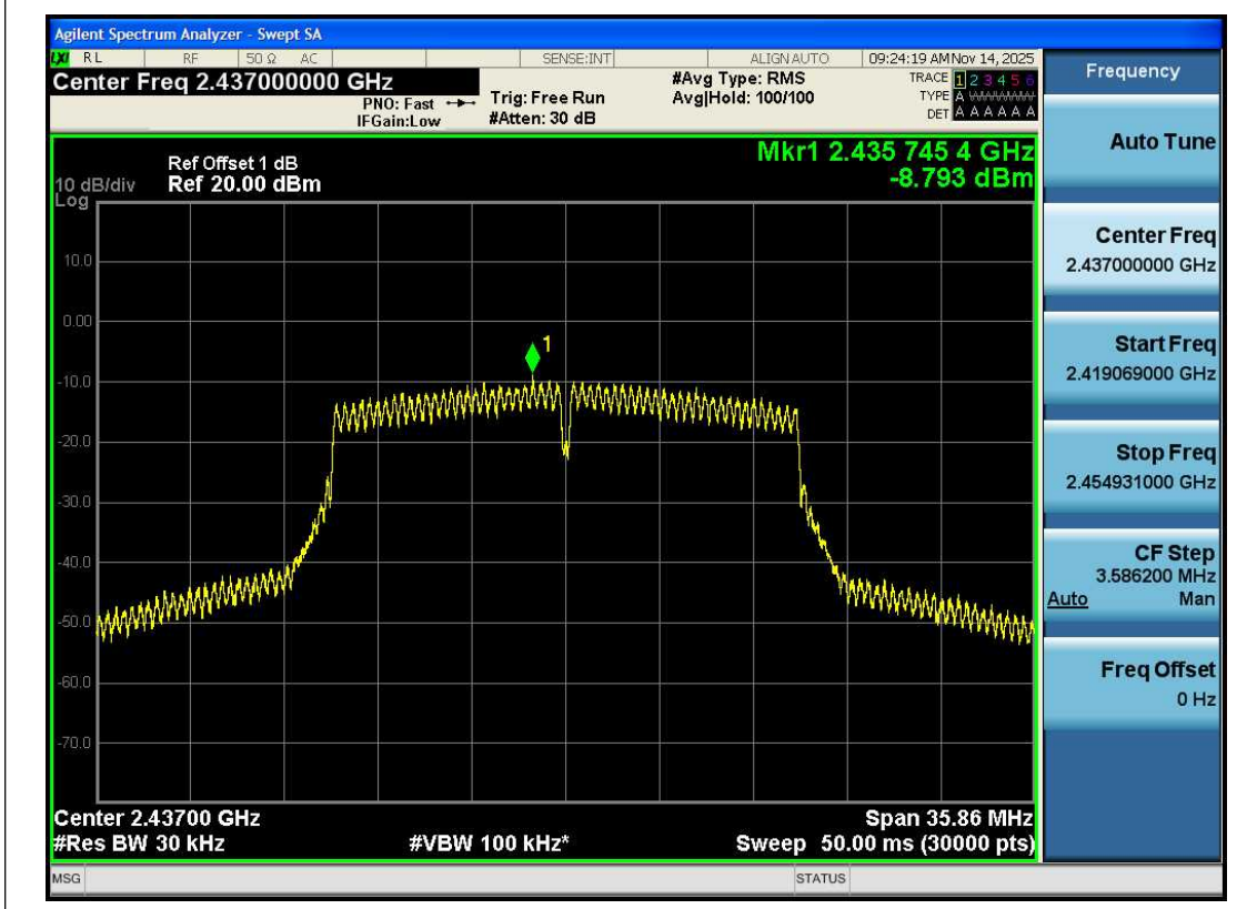
11N20SISO-Ant1-2437-PASS
