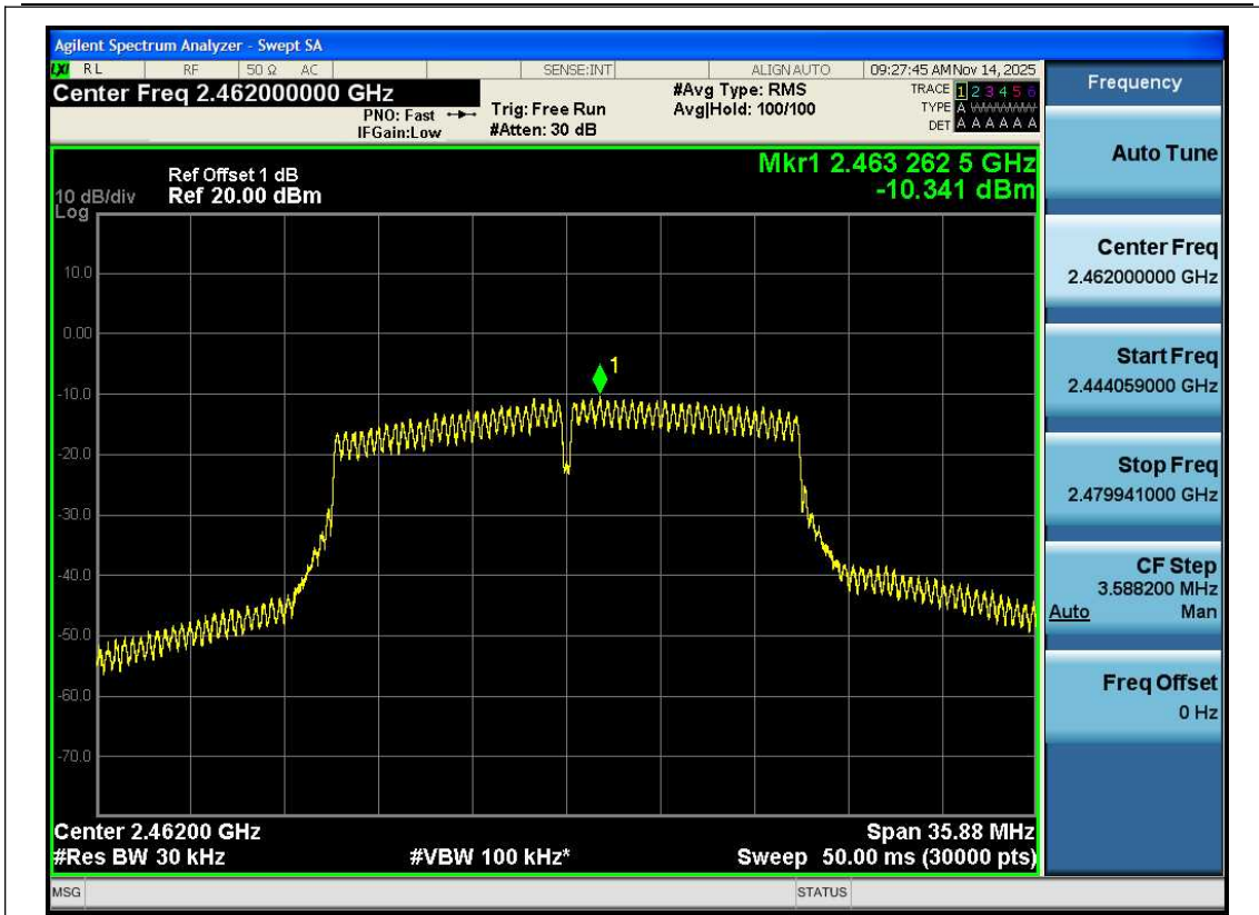
11N20SISO-Ant1-2462-PASS
