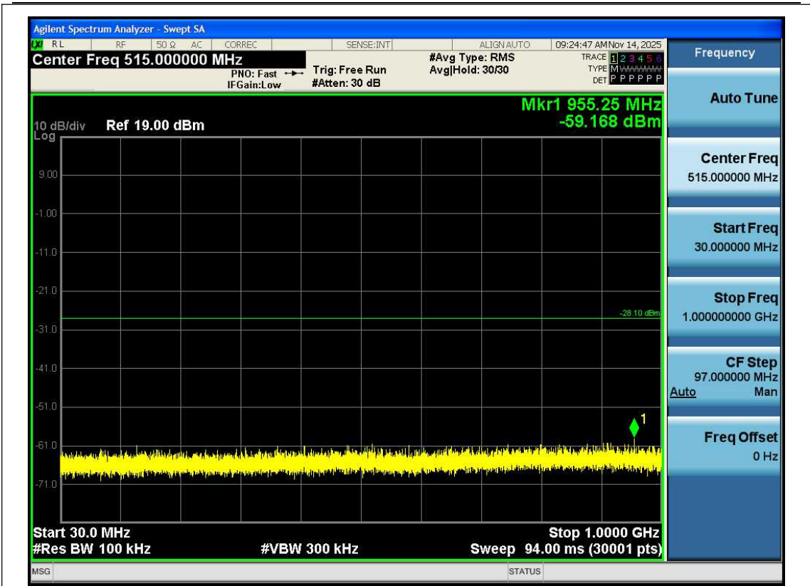
11N20SISO-Ant1-2437-30~1000-PASS
