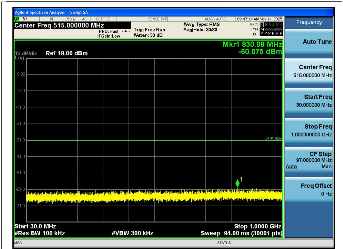
11N40SISO-Ant1-2452-30~1000-PASS
