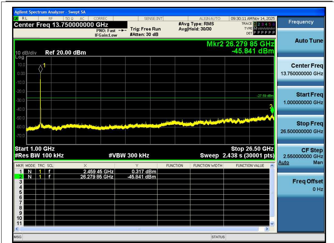
11N20SISO-Ant1-2462-1000~26500-PASS
