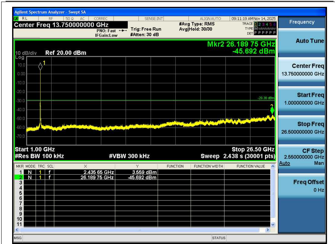
11G-Ant1-2437-1000~26500-PASS
