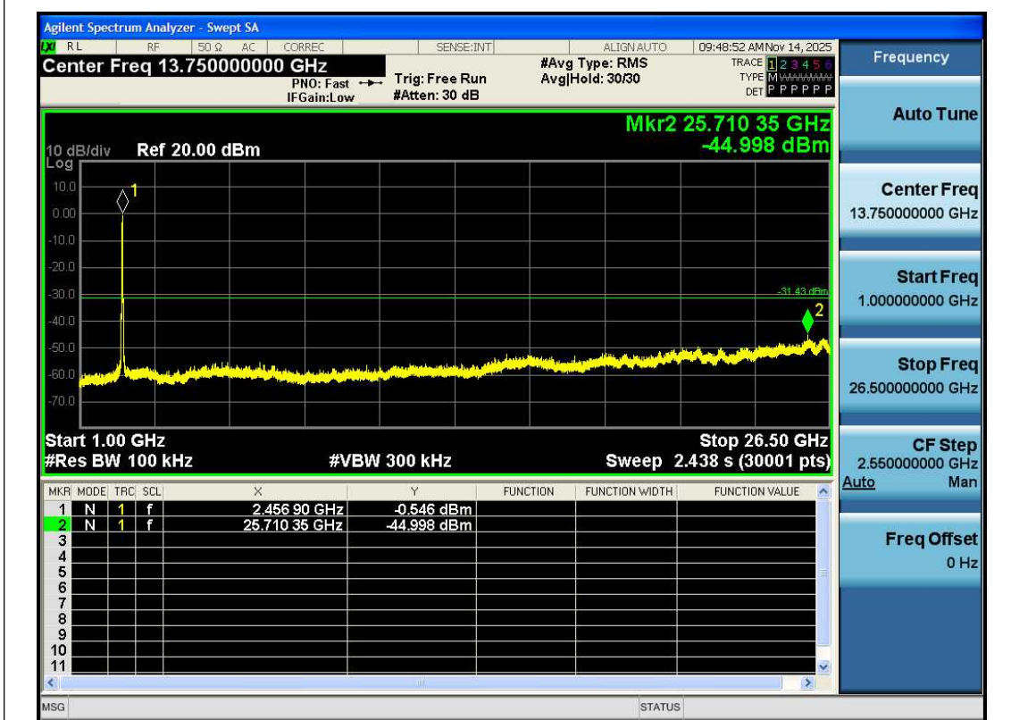
11N40SISO-Ant1-2452-1000~26500-PASS
