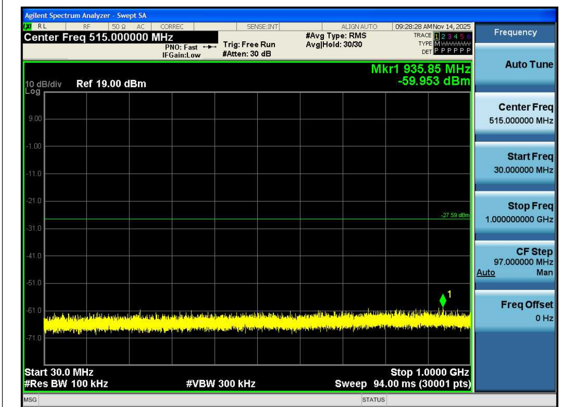
11N20SISO-Ant1-2462-30~1000-PASS
