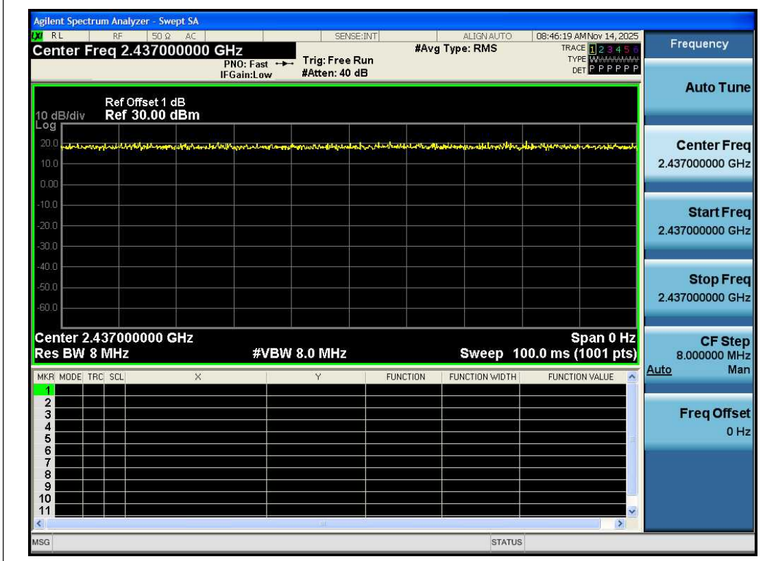
NTNV-11N20SISO-Ant1-2437
