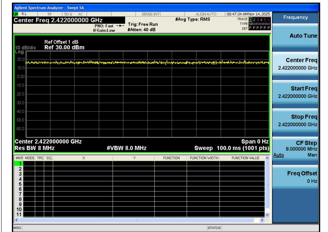
NTNV-11N40SISO-Ant1-2422
