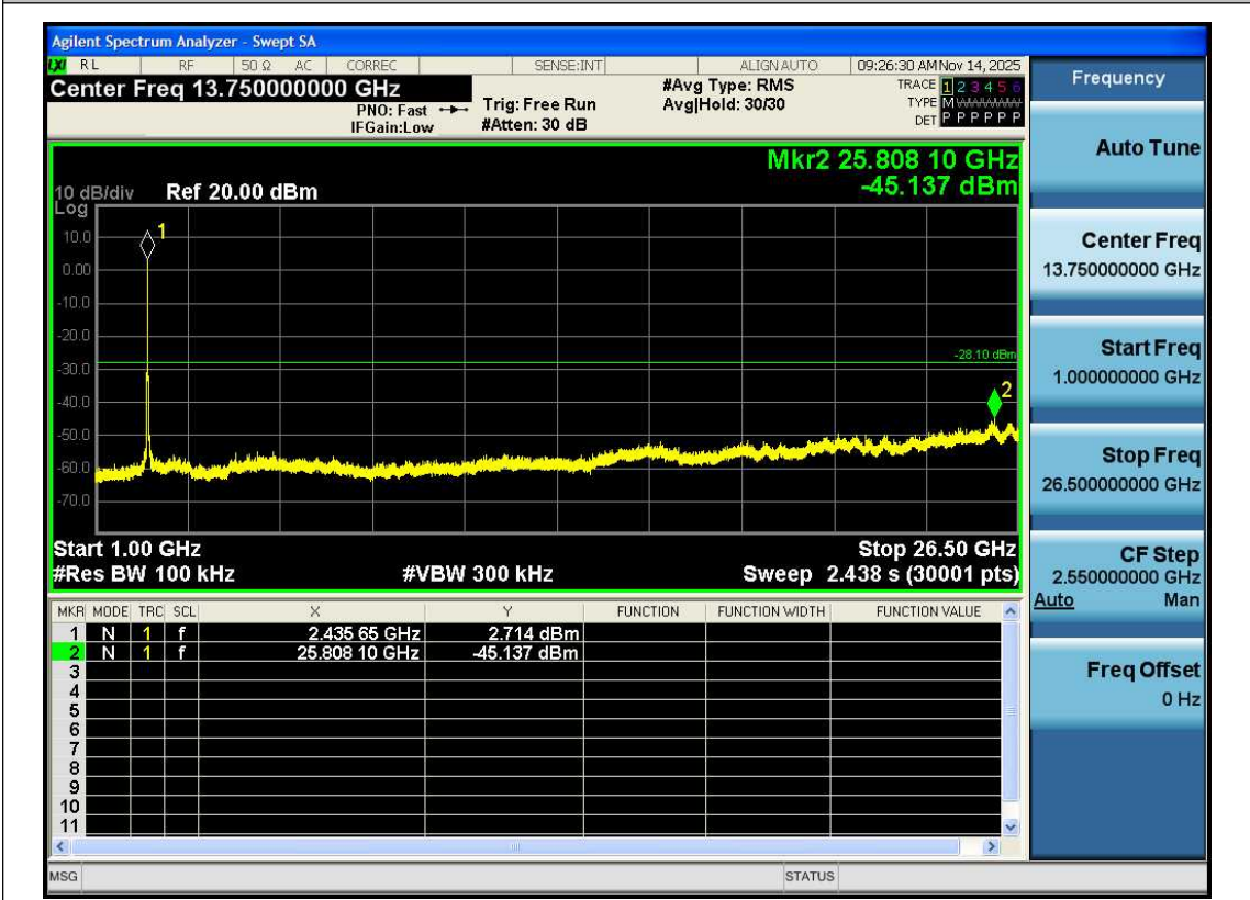
11N20SISO-Ant1-2437-1000~26500-PASS
