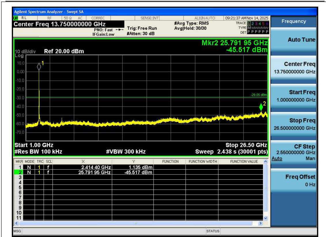
11N20SISO-Ant1-2412-1000~26500-PASS
