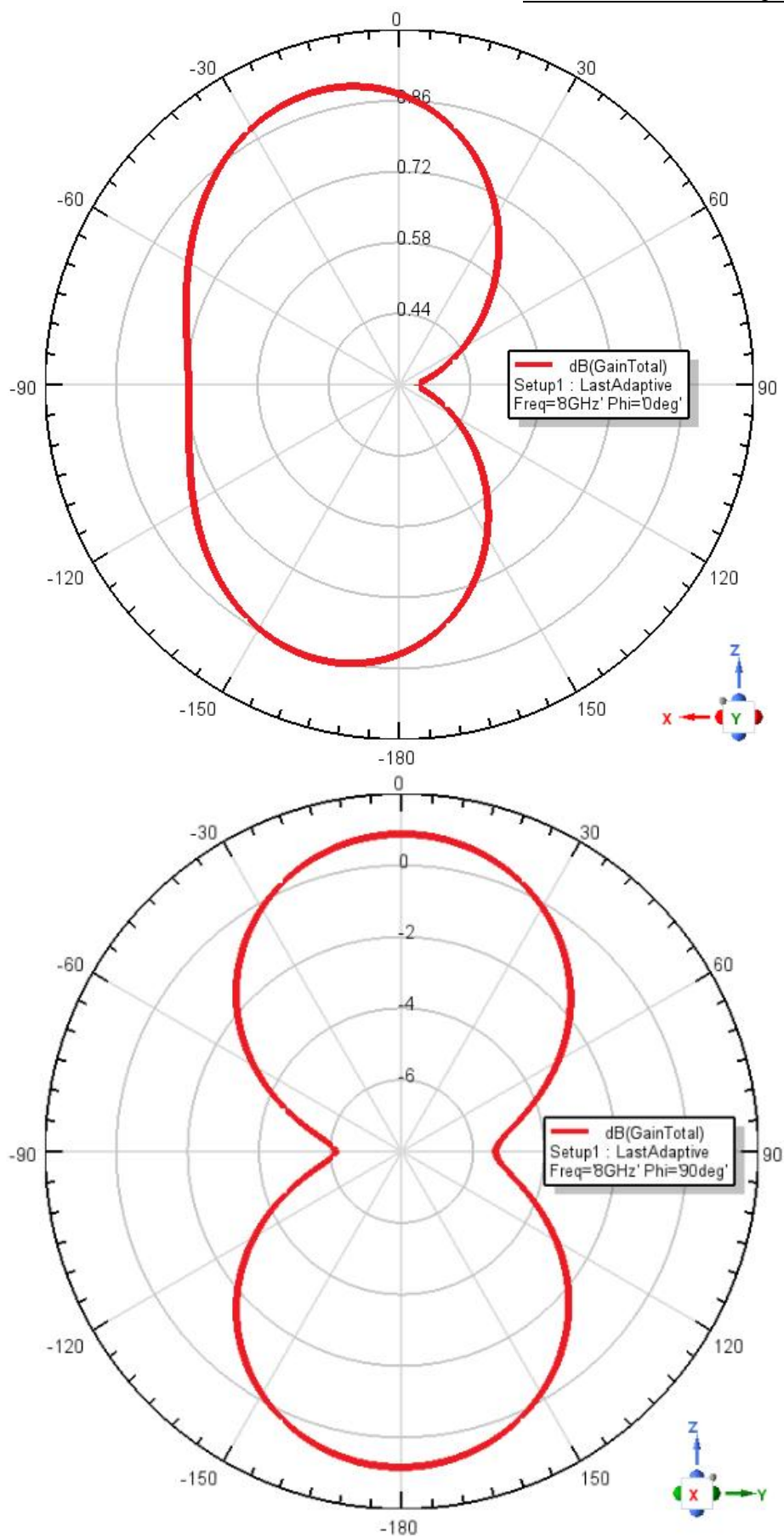
Figure 5 8GHz 2D Antenna Pattern
