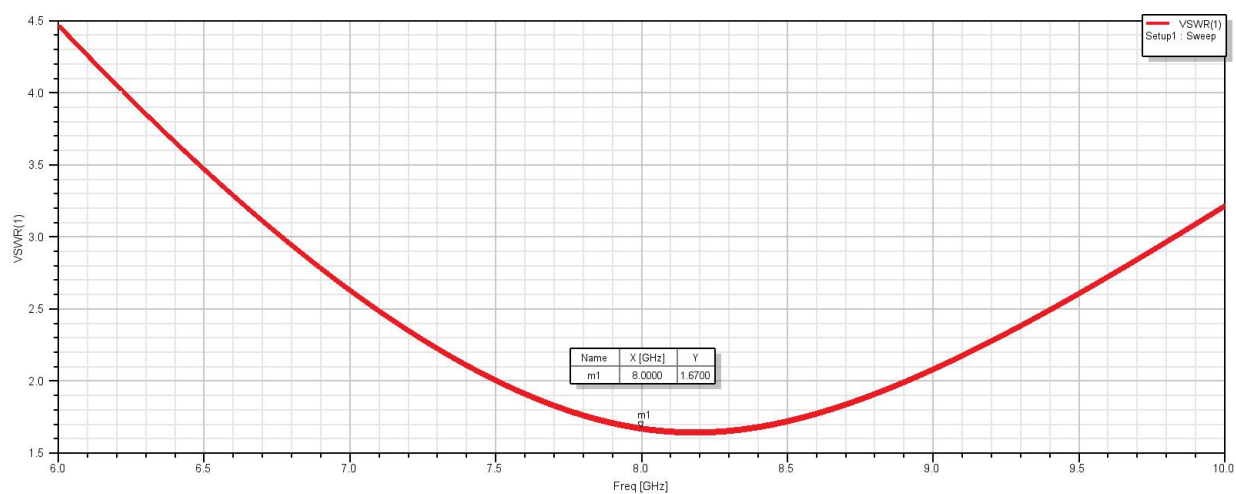
Figure 3 Voltage Standing Wave Ratio
