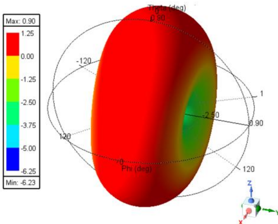
Figure 4 8GHz 3D Antenna Pattern
