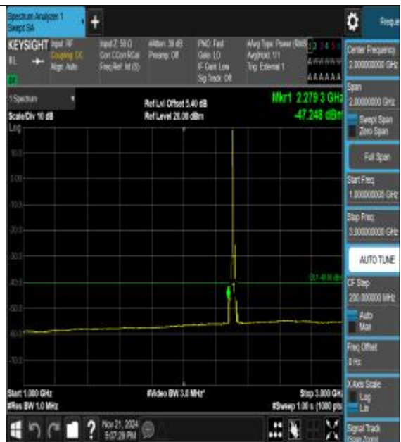
Band40_10MHz_QPSK_38750_1RB#0_1000~3000_0_1000~3000
