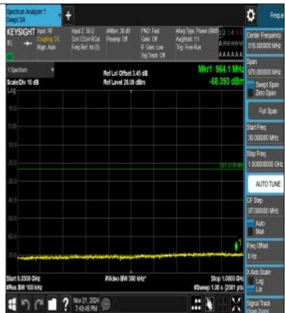
Band66_1.4MHz_16QAM_132665_1RB#0_30~1000_30~1000
