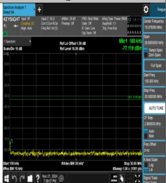
Band66_1.4MHz_QPSK_131979_1RB#0_0.15~30_0.15~30
