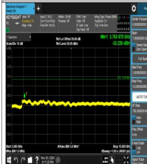
Band26_5MHz_QPSK_26765_1RB#0_3000~10000_3000~10000
