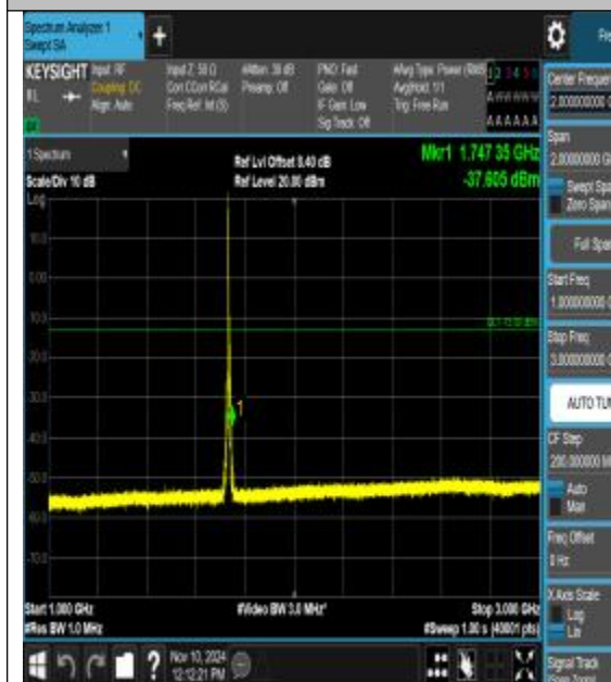
Band4_5MHz_16QAM_20175_1RB#0_1000~300_0_1000~3000
