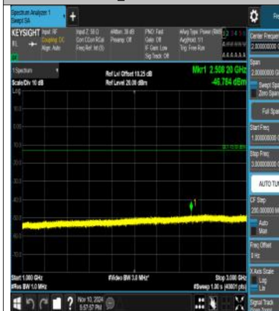
Band5_1.4MHz_16QAM_20525_1RB#0_1000~3000_1000~3000
