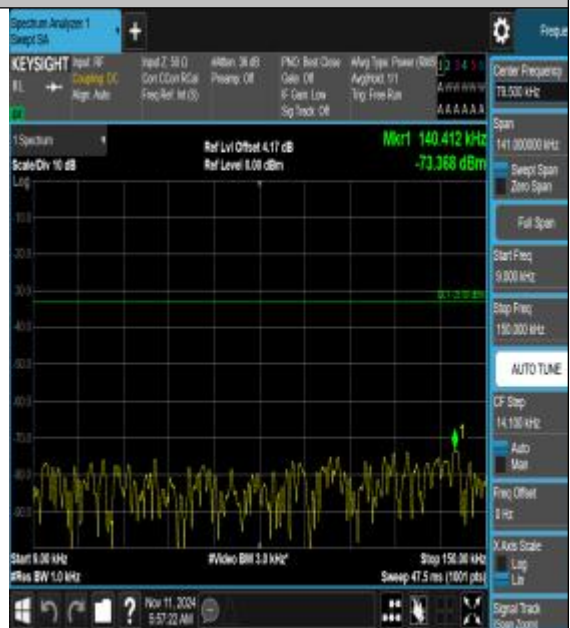
Band5_10MHz_16QAM_20450_1RB#0_0.009~0.15_0.009~0.15
