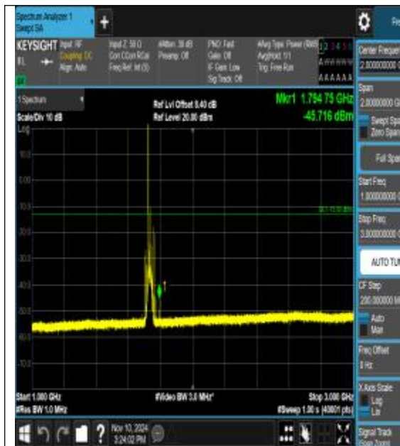
Band4_20MHz_16QAM_20175_1RB#0_1000~3000_1000~3000
