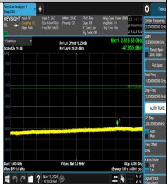
Band5_10MHz_QPSK_20525_1RB#0_1000~3000 _1000~3000
