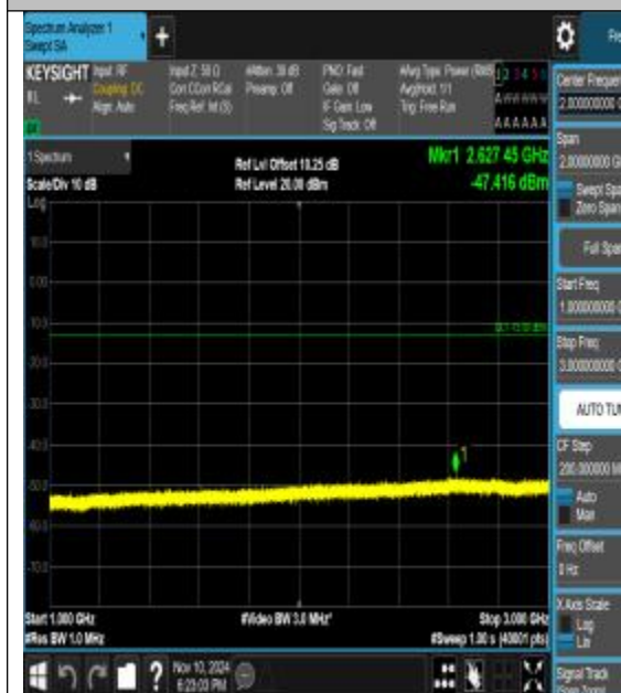
Band5_3MHz_16QAM_20635_1RB#0_1000~300_0_1000~3000
