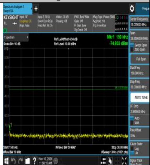
Band4_3MHz_QPSK_20385_1RB#0_0.15~30_0.15~30_5~30
