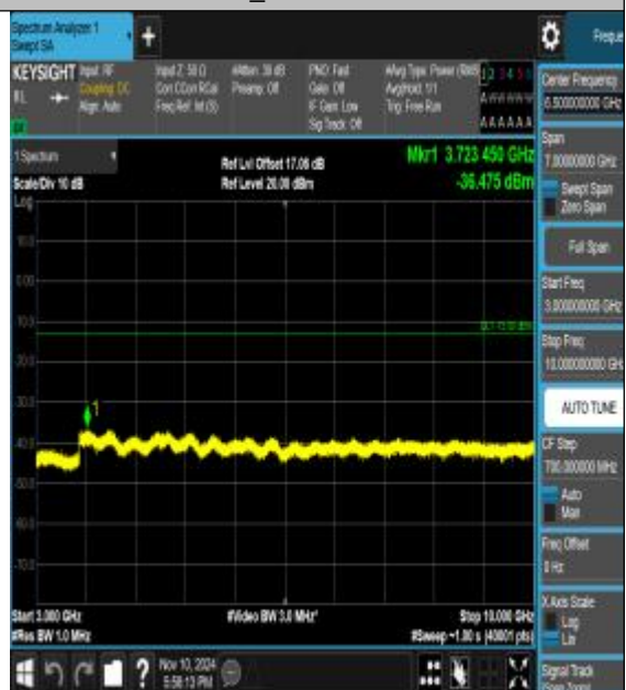
Band5_1.4MHz_16QAM_20525_1RB#0_3000~10000_3000~10000
