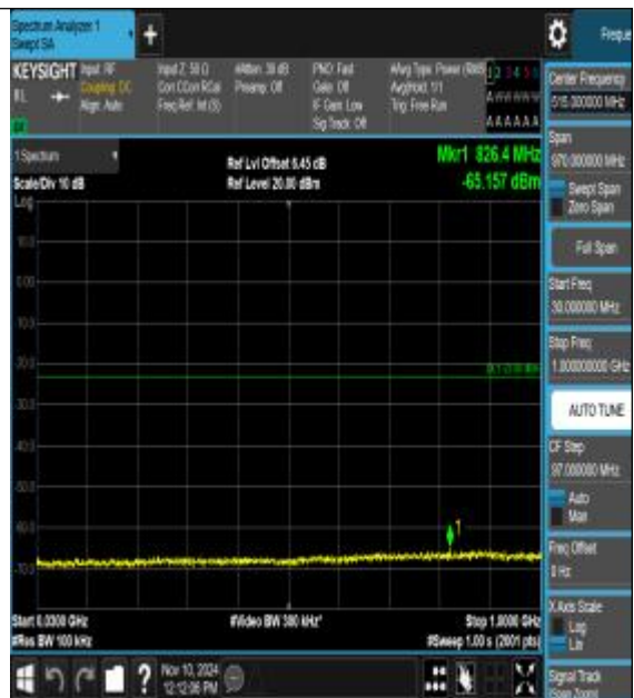
Band4_5MHz_16QAM_20175_1RB#0_30~1000_0~1000
