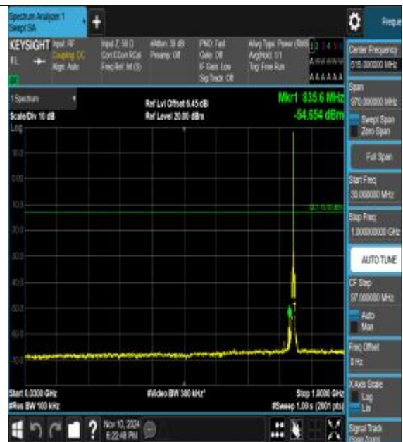
Band5_3MHz_16QAM_20635_1RB#0_30~1000_30~1000
