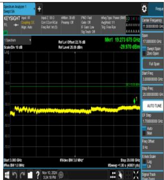
Band4_20MHz_16QAM_20175_1RB#0_3000~20000_3000~20000
