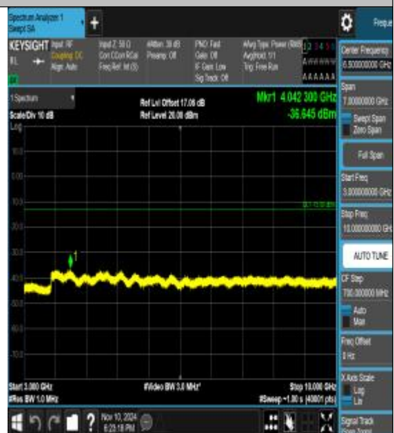
Band5_3MHz_16QAM_20635_1RB#0_3000~1000_0_3000~10000
