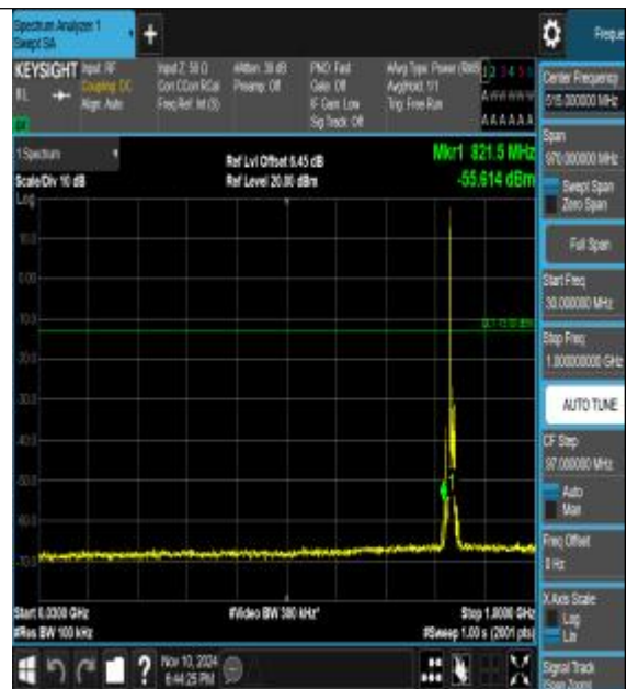
Band5_5MHz_16QAM_20525_1RB#0_30~1000_30~1000
