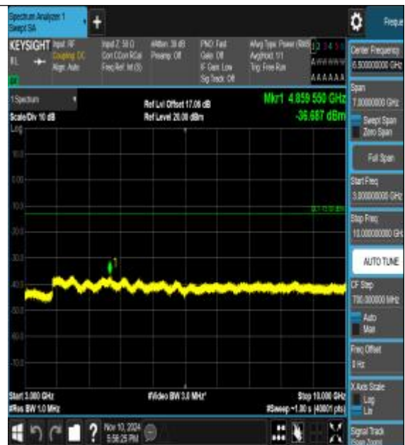
Band5_1.4MHz_16QAM_20407_1RB#0_3000~10000_000_3000~10000
