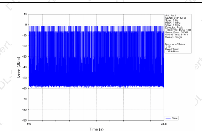
2-DH1
