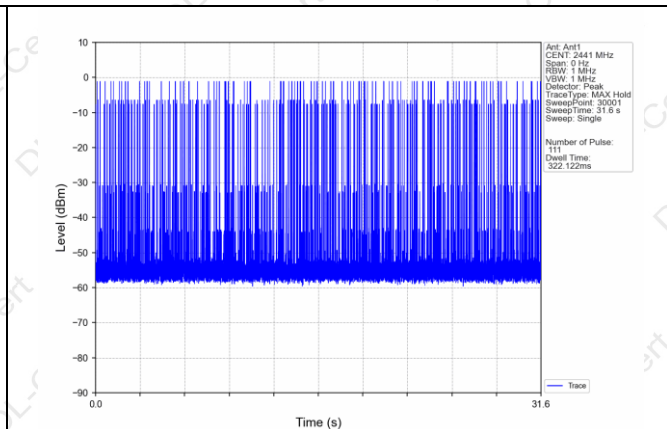
2-DH3
