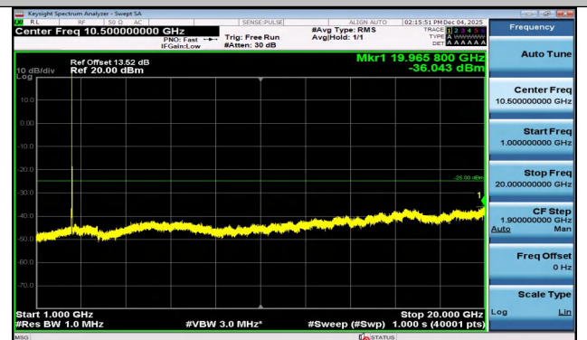
Band7-10MHz-QPSK-20800-1RB#0-1000~20000-PASS
