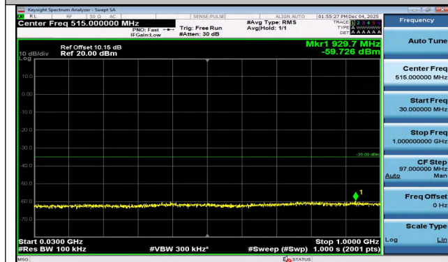
Band7-5MHz-QPSK-21425-25RB#0-30~1000-PASS
