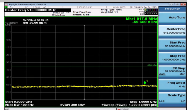
Band7-5MHz-16QAM-21425-1RB#0-30~1000-PASS
