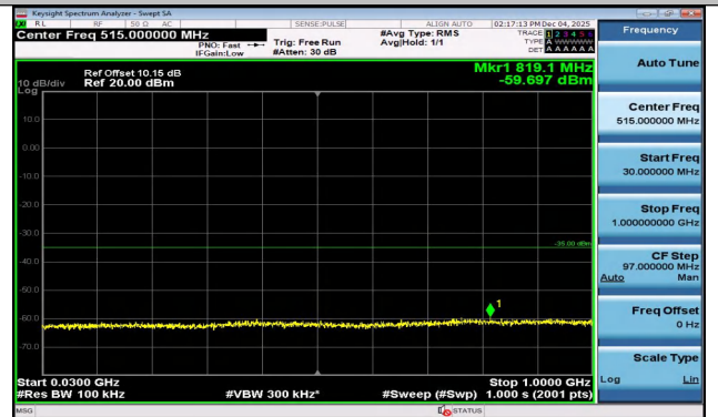
Band7-10MHz-QPSK-20800-1RB#49-30~1000-PASS
