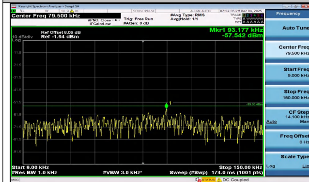
Band7-10MHz-QPSK-20800-1RB#0-0.009~0.15-PASS
