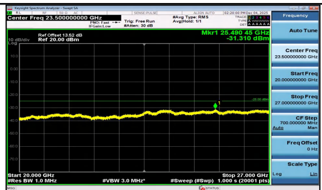
Band7-10MHz-16QAM-20800-50RB#0-20000~27000-PAS
