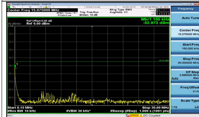
Band7-10MHz-16QAM-20800-1RB#0-0.15~30-PASS
