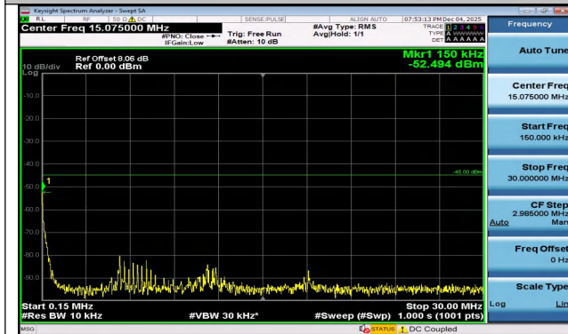
Band7-10MHz-QPSK-20800-1RB#49-0.15~30-PASS
