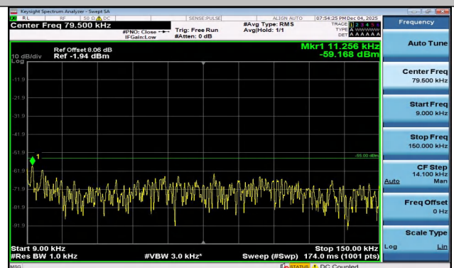
Band7-10MHz-QPSK-21100-1RB#49-0.009~0.15-PASS
