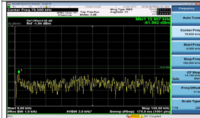
Band7-5MHz-16QAM-21425-1RB#24-0.009~0.15-PASS
