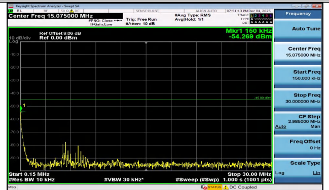
Band7-5MHz-16QAM-21425-1RB#24-0.15~30-PASS
