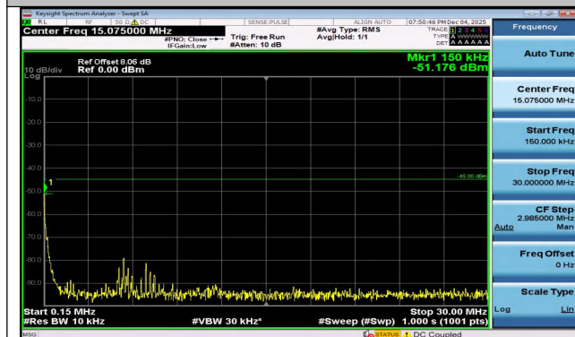
Band7-5MHz-16QAM-21425-1RB#0-0.15~30-PASS
