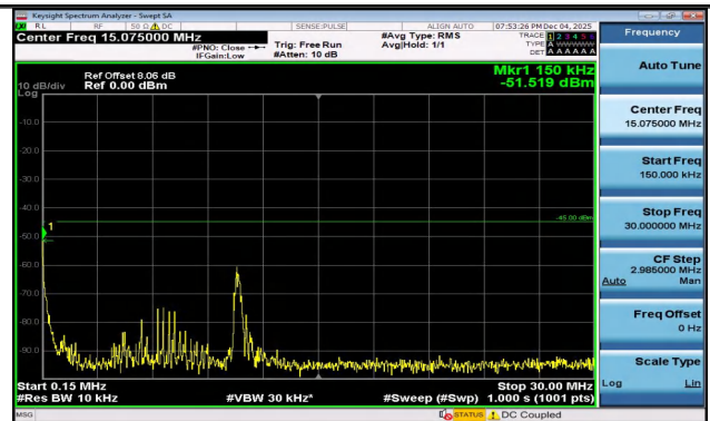
Band7-10MHz-16QAM-20800-1RB#49-0.15~30-PASS
