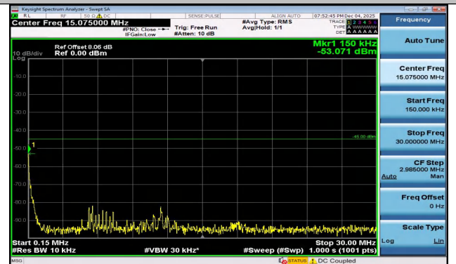
Band7-10MHz-QPSK-20800-1RB#0-0.15~30-PASS
