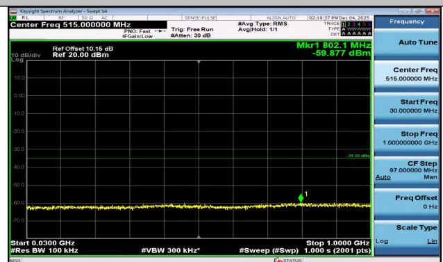
Band7-10MHz-16QAM-20800-50RB#0-30~1000-PASS
