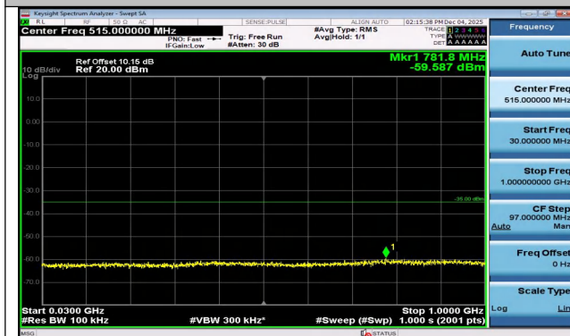
Band7-10MHz-QPSK-20800-1RB#0-30~1000-PASS
