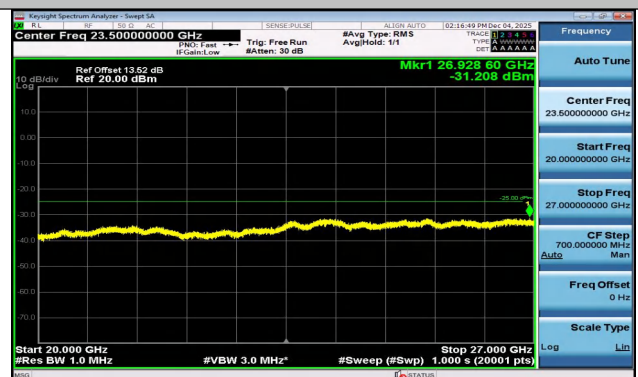
Band7-10MHz-16QAM-20800-1RB#0-20000~27000-PASS
