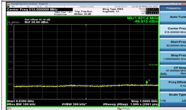
Band7-5MHz-16QAM-21425-1RB#24-30~1000-PASS
