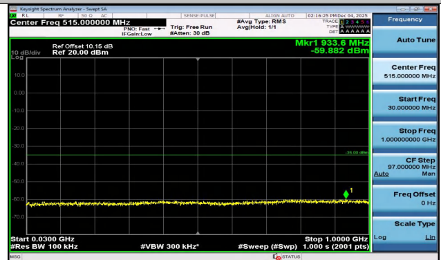
Band7-10MHz-16QAM-20800-1RB#0-30~1000-PASS
