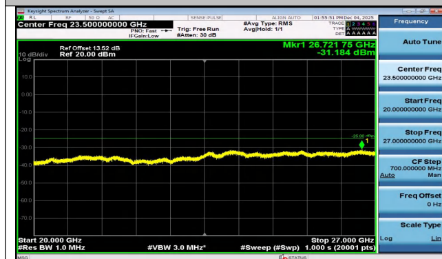
Band7-5MHz-QPSK-21425-25RB#0-20000~27000-PASS
