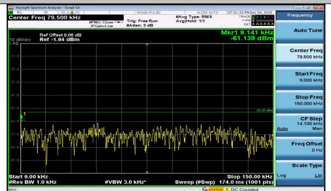
Band7-5MHz-16QAM-21425-25RB#0-0.009~0.15-PASS
