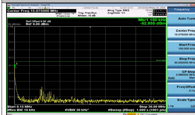
Band7-10MHz-16QAM-20800-50RB#0-0.15~30-PASS
