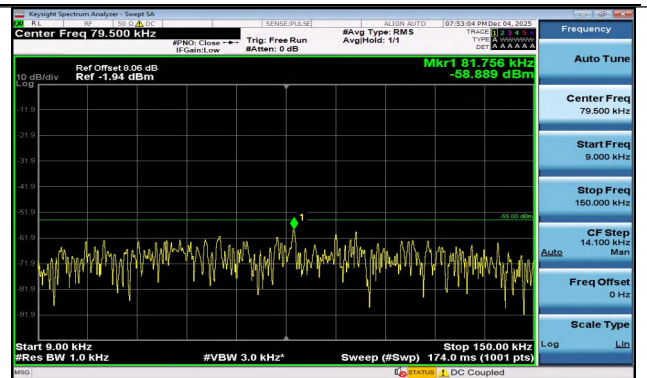
Band7-10MHz-QPSK-20800-1RB#49-0.009~0.15-PASS
