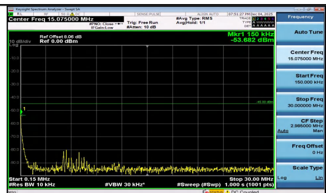
Band7-5MHz-QPSK-21425-25RB#0-0.15~30-PASS
