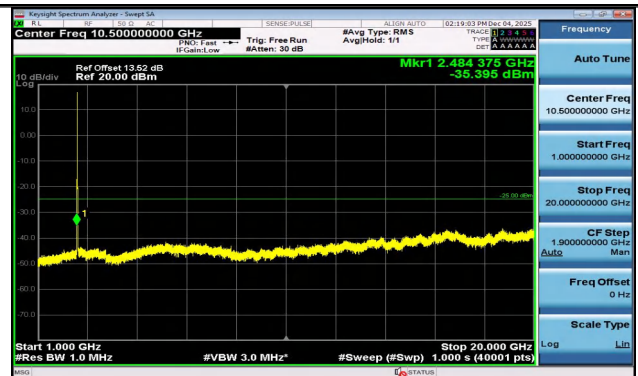
Band7-10MHz-QPSK-20800-50RB#0-1000~20000-PASS
