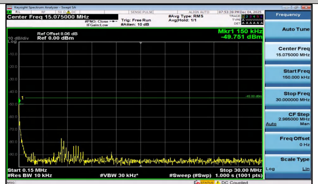
Band7-10MHz-QPSK-20800-50RB#0-0.15~30-PASS
