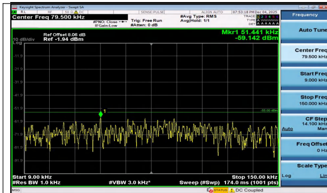
Band7-10MHz-16QAM-20800-1RB#49-0.009~0.15-PASS
