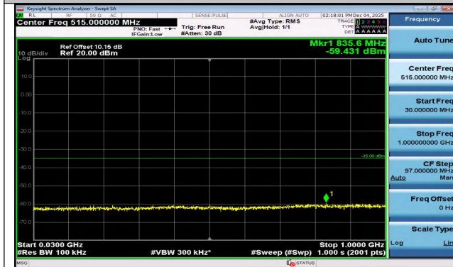
Band7-10MHz-16QAM-20800-1RB#49-30~1000-PASS
