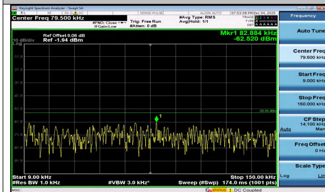
Band7-10MHz-QPSK-21100-1RB#0-0.009~0.15-PASS
