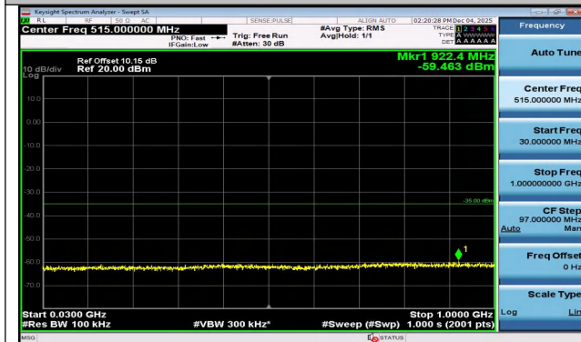
Band7-10MHz-QPSK-21100-1RB#0-30~1000-PASS
