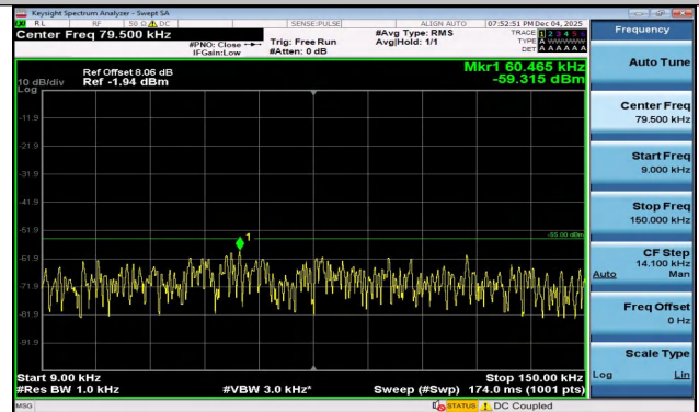
Band7-10MHz-16QAM-20800-1RB#0-0.009~0.15-PASS
