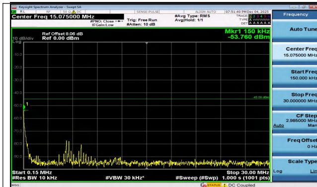
Band7-5MHz-16QAM-21425-25RB#0-0.15~30-PASS
