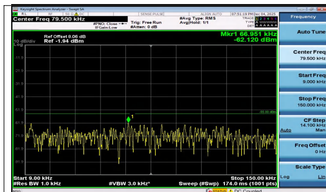
Band7-5MHz-QPSK-21425-25RB#0-0.009~0.15-PASS
