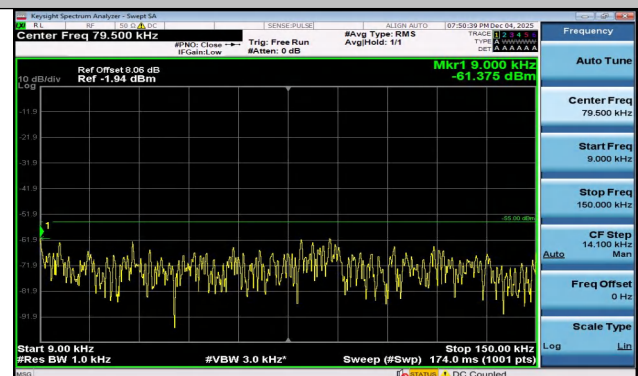
Band7-5MHz-16QAM-21425-1RB#0-0.009~0.15-PASS
