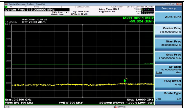
Band7-5MHz-16QAM-21425-25RB#0-30~1000-PASS
