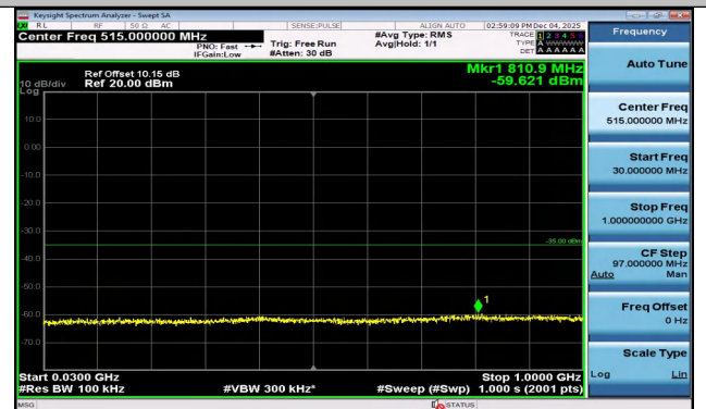
Band7-15MHz-16QAM-21375-1RB#0-30~1000-PASS
