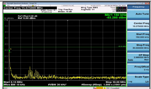
Band7-15MHz-QPSK-21375-1RB#0-0.15~30-PASS
