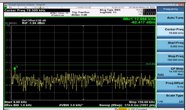
Band7-15MHz-QPSK-21375-1RB#74-0.009~0.15-PASS
