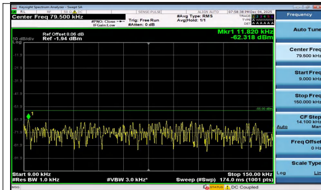
Band7-15MHz-16QAM-21100-1RB#74-0.009~0.15-PASS
