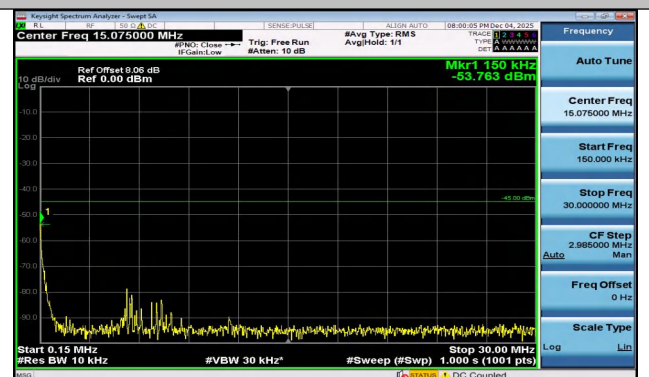
Band7-15MHz-16QAM-21375-1RB#74-0.15~30-PASS
