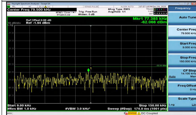
Band7-15MHz-16QAM-20825-1RB#74-0.009~0.15-PASS
