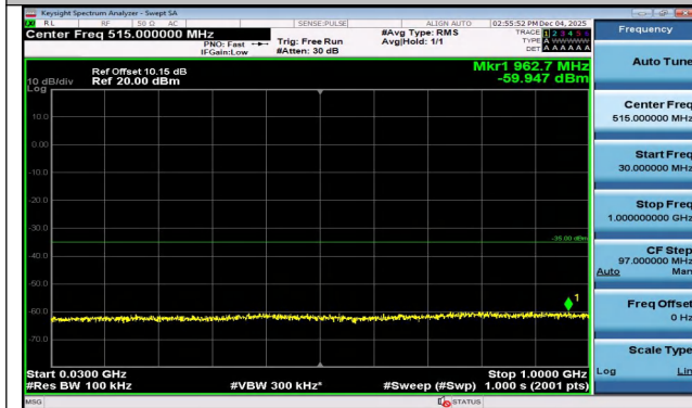
Band7-15MHz-16QAM-21100-1RB#74-30~1000-PASS
