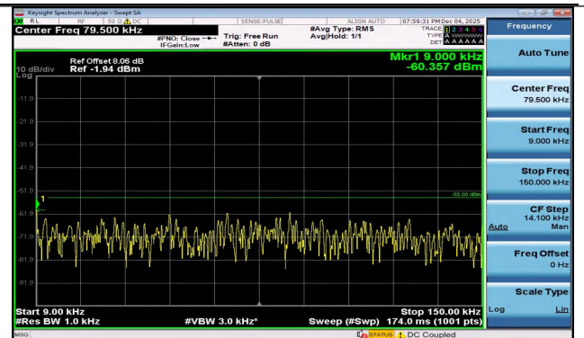
Band7-15MHz-16QAM-21375-1RB#0-0.009~0.15-PASS
