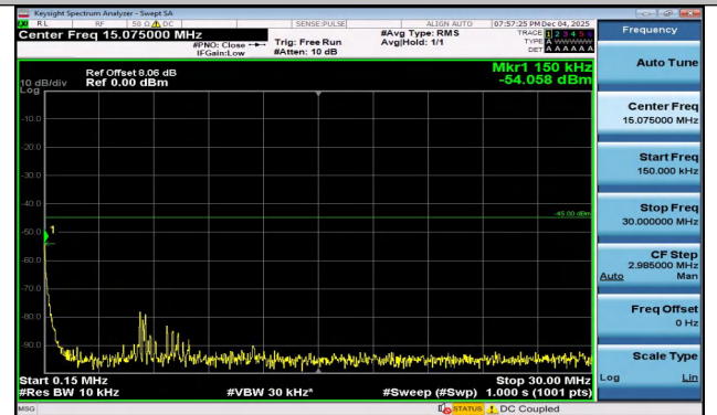
Band7-15MHz-16QAM-20825-1RB#74-0.15~30-PASS
