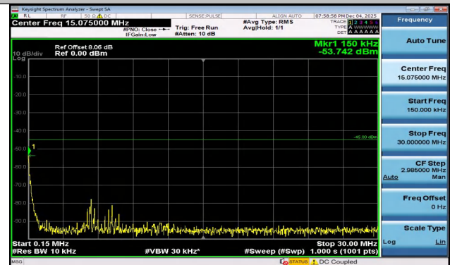
Band7-15MHz-QPSK-21100-75RB#0-0.15~30-PASS
