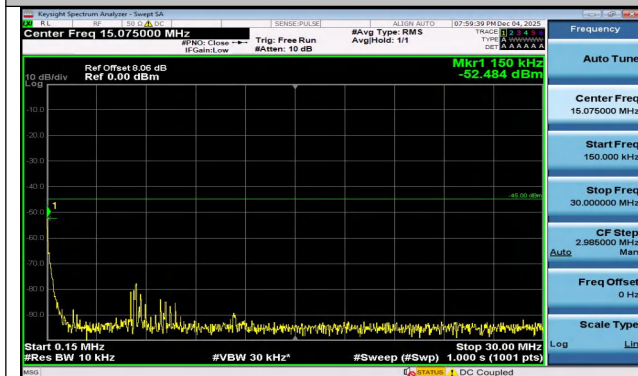
Band7-15MHz-16QAM-21375-1RB#0-0.15~30-PASS
