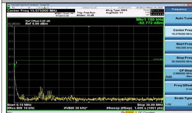
Band7-15MHz-16QAM-21100-75RB#0-0.15~30-PASS
