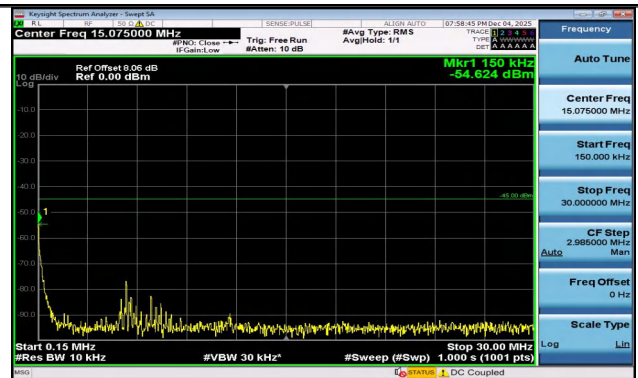
Band7-15MHz-16QAM-21100-1RB#74-0.15~30-PASS
