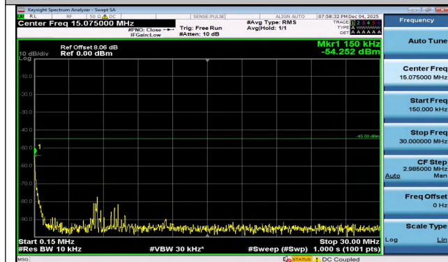
Band7-15MHz-QPSK-21100-1RB#74-0.15~30-PASS
