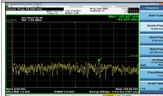
Band7-15MHz-16QAM-21375-1RB#74-0.009~0.15-PASS
