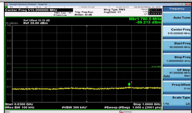
Band7-15MHz-QPSK-21100-1RB#74-30~1000-PASS
