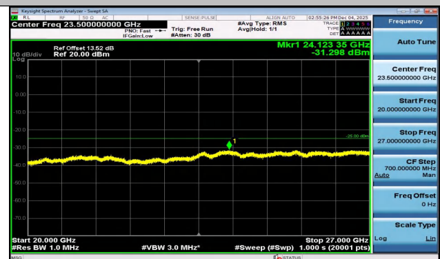
Band7-15MHz-QPSK-21100-1RB#74-20000~27000-PASS
