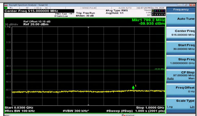
Band7-15MHz-16QAM-21100-75RB#0-30~1000-PASS
