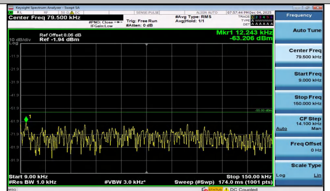
Band7-15MHz-16QAM-20825-75RB#0-0.009~0.15-PASS
