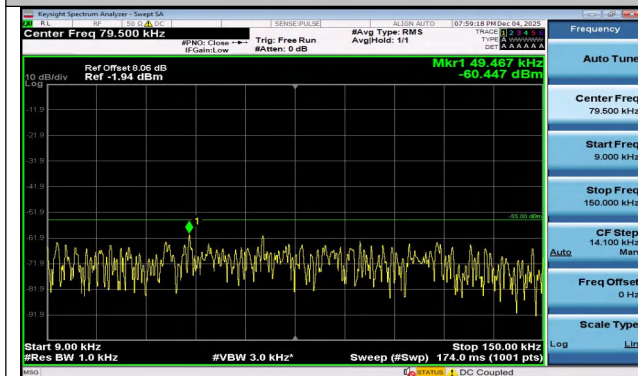
Band7-15MHz-QPSK-21375-1RB#0-0.009~0.15-PASS
