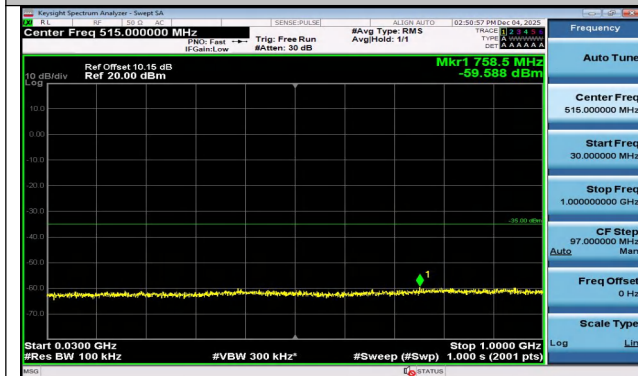
Band7-15MHz-16QAM-20825-1RB#74-30~1000-PASS
