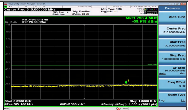
Band7-15MHz-16QAM-21375-75RB#0-30~1000-PASS
