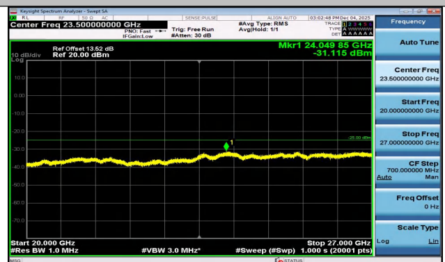
Band7-15MHz-16QAM-21375-75RB#0-20000~27000-PASS
