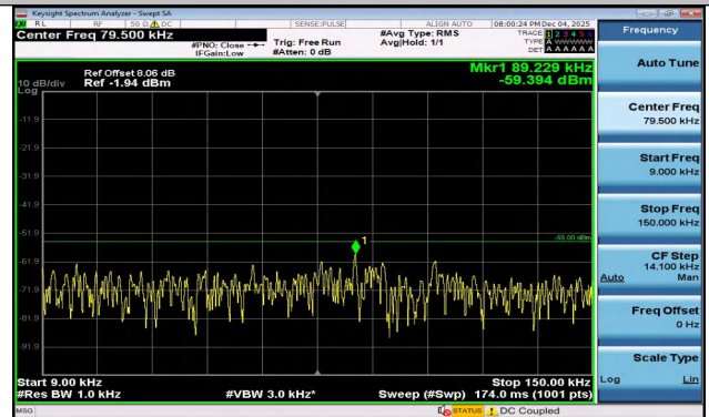
Band7-15MHz-16QAM-21375-75RB#0-0.009~0.15-PASS
