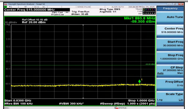
Band7-20MHz-16QAM-20850-100RB#0-30~1000-PASS
