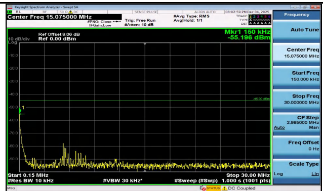
Band7-20MHz-QPSK-21100-100RB#0-0.15~30-PASS
