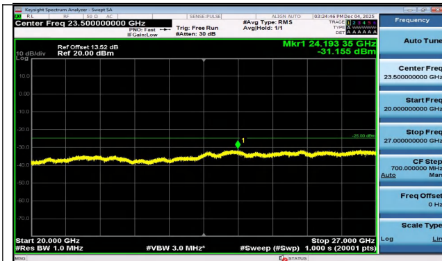
Band7-20MHz-16QAM-20850-1RB#99-20000~27000-PA SS
