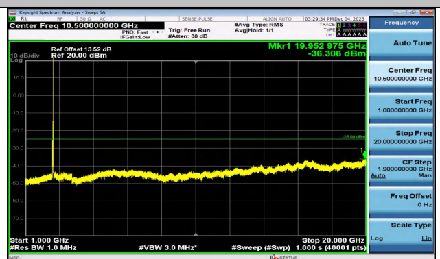
Band7-20MHz-16QAM-21100-1RB#99-1000~20000-PASS
