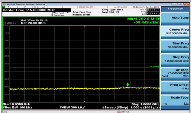
Band7-20MHz-QPSK-21100-1RB#99-30~1000-PASS
