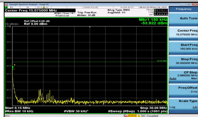
Band7-20MHz-QPSK-21100-1RB#99-0.15~30-PASS
