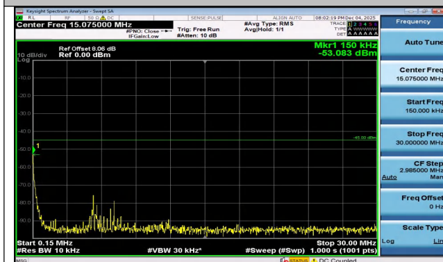
Band7-20MHz-16QAM-21100-1RB#0-0.15~30-PASS
