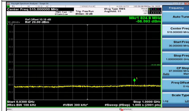
Band7-20MHz-QPSK-21100-100RB#0-30~1000-PASS
