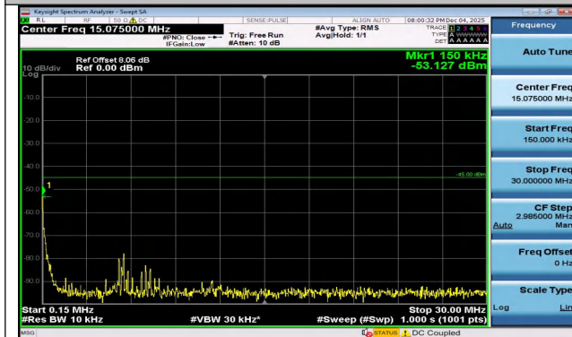
Band7-15MHz-16QAM-21375-75RB#0-0.15~30-PASS
