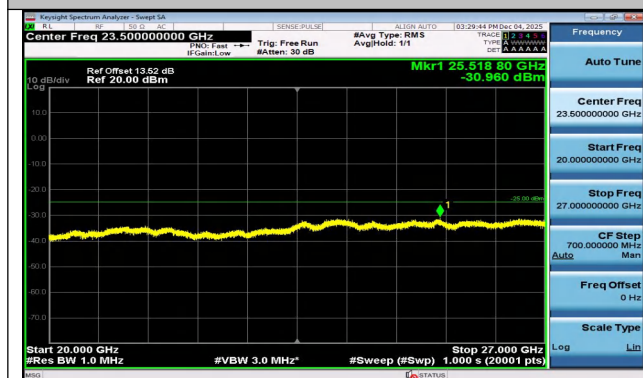
Band7-20MHz-16QAM-21100-1RB#99-20000~27000-PAS
