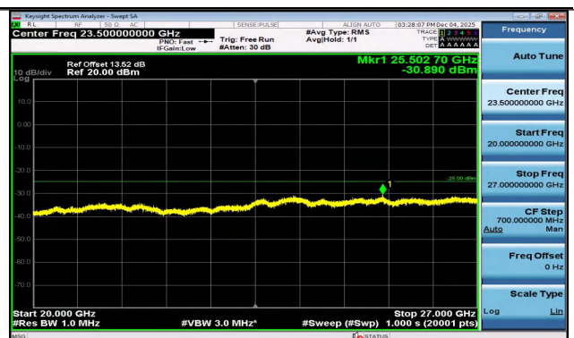
Band7-20MHz-16QAM-21100-1RB#0-20000~27000-PASS
