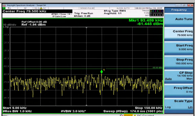
Band7-20MHz-QPSK-21100-1RB#99-0.009~0.15-PASS
