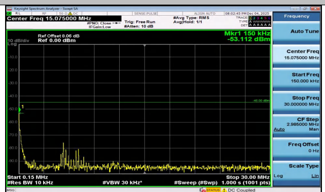
Band7-20MHz-16QAM-21100-1RB#99-0.15~30-PASS
