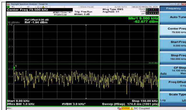
Band7-20MHz-QPSK-21100-100RB#0-0.009~0.15-PASS
