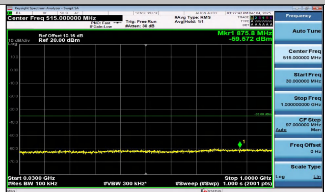
Band7-20MHz-16QAM-21100-1RB#0-30~1000-PASS
