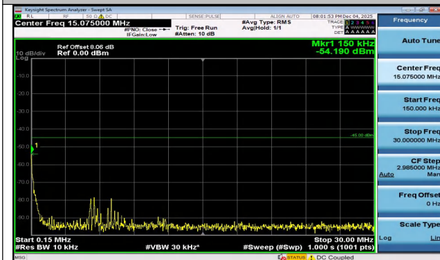
Band7-20MHz-16QAM-20850-100RB#0-0.15~30-PASS
