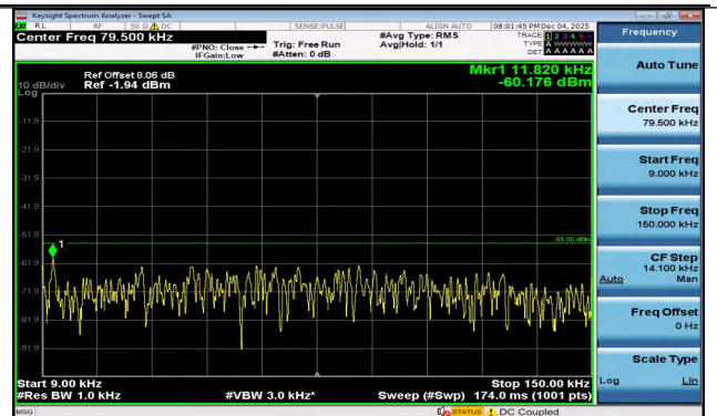
Band7-20MHz-16QAM-20850-100RB#0-0.009~0.15-PASS
