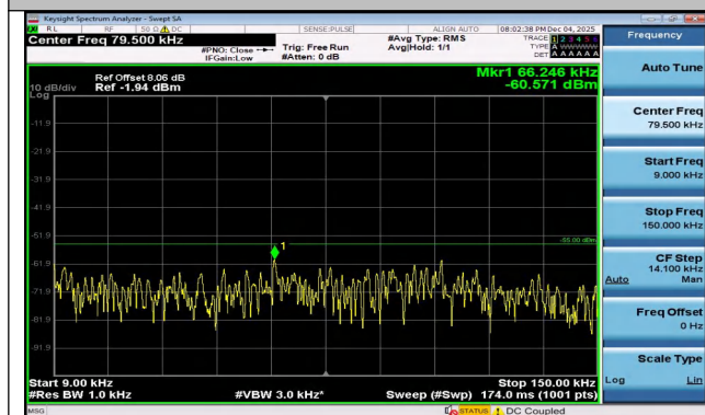
Band7-20MHz-16QAM-21100-1RB#99-0.009~0.15-PASS
