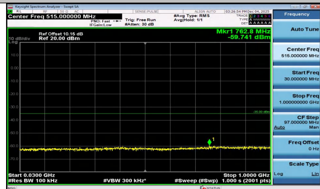
Band7-20MHz-QPSK-21100-1RB#0-30~1000-PASS
