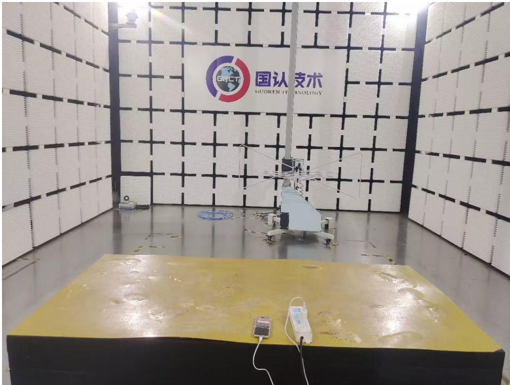
Fig.3 appearance 3
