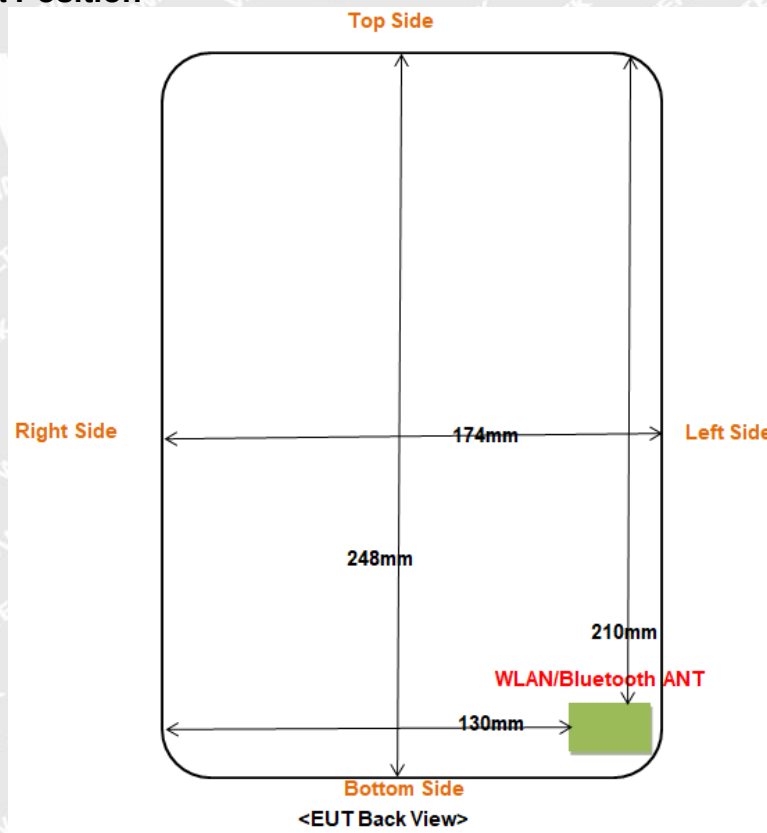
Fig 7.2 Block Diagram for EUT Antenna Position
