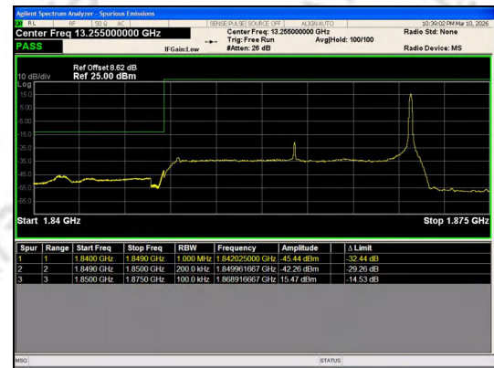
Band 25 20MHz/1860.0/Low QPSK 100@0
