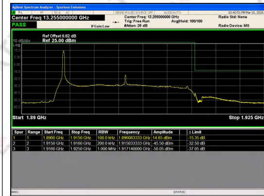
Band 25 20MHz/1905.0/High QPSK 1@99
