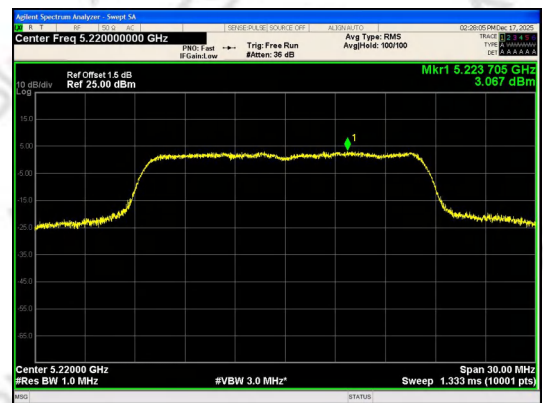
IEEE 802.11a_Channel 44_20MHz_Antenna 0
