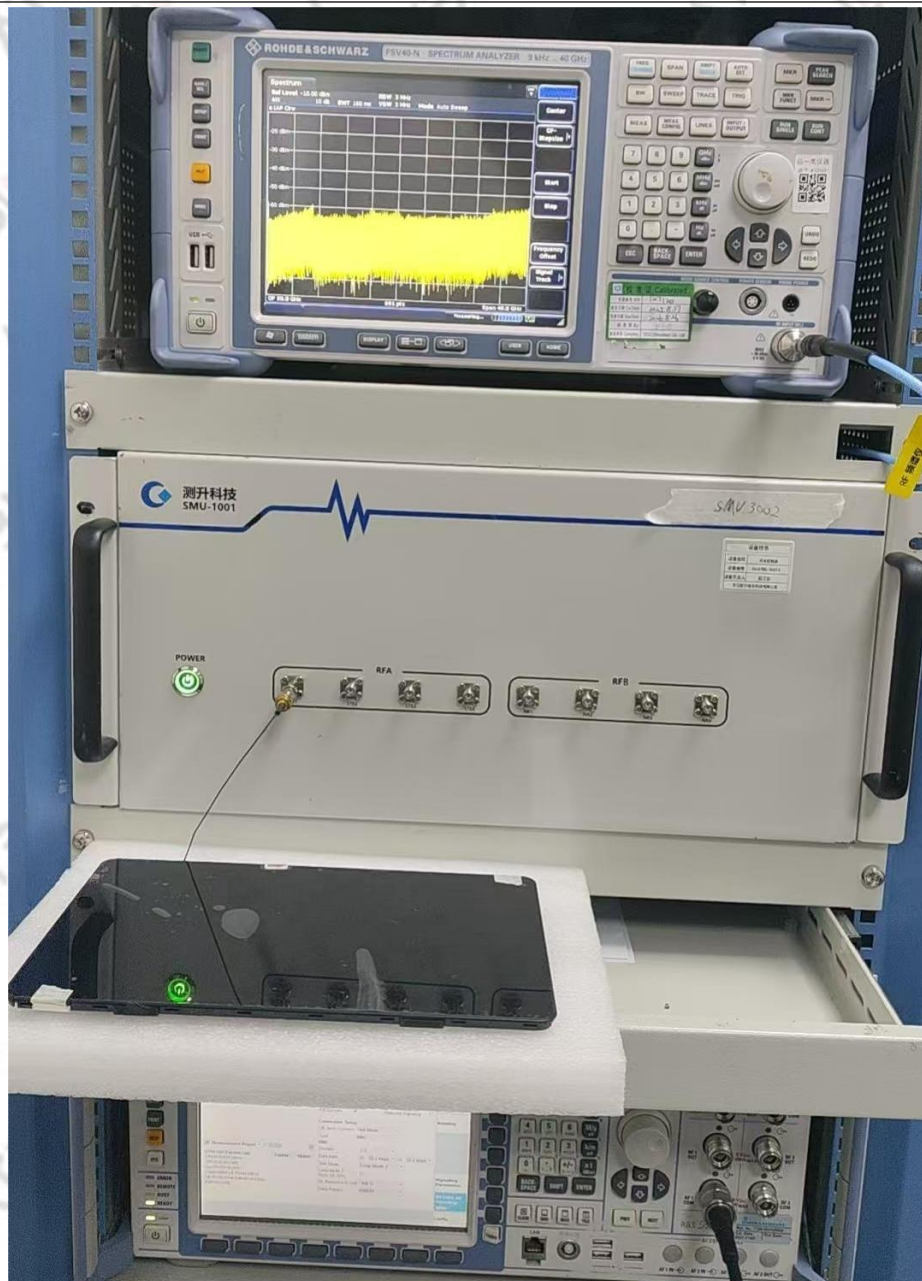
Conducted test photos 2
