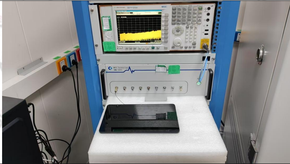
2/3/4G_Conducted test photos
