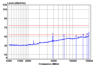
BLE_1M_TX_CH_19_Horizontal
