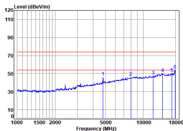
BLE_1M_TX_CH_00_Vertical
