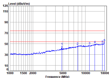
BLE_1M_TX_CH_19_Vertical
