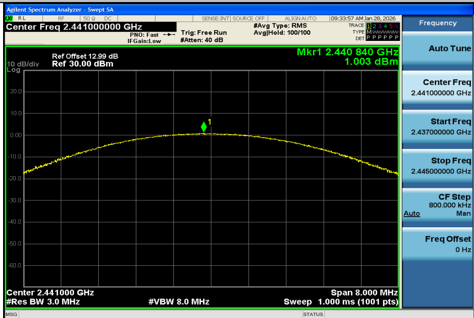
2DH5-Ant1-2441-PASS
