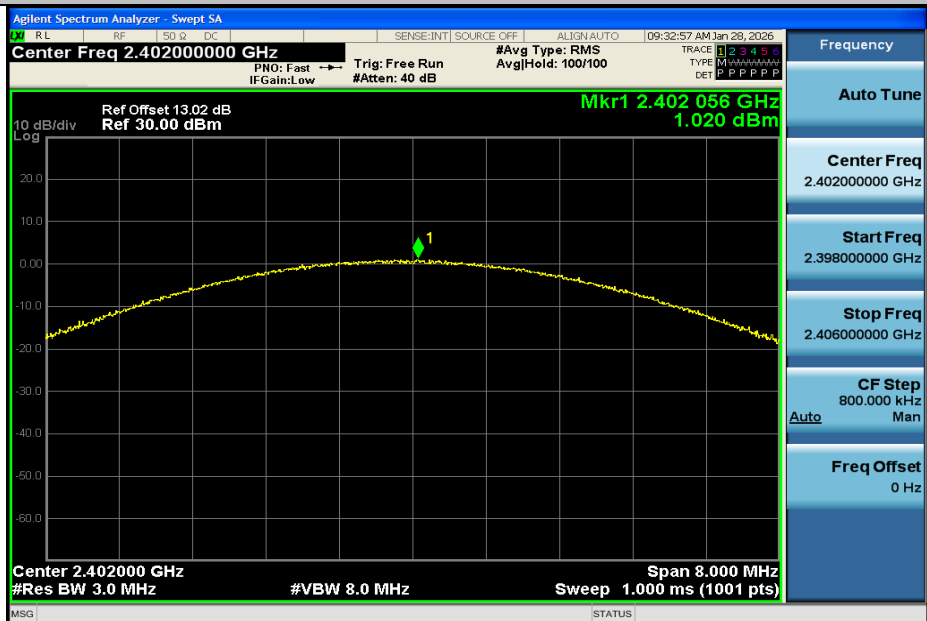
3DH5-Ant1-2402-PASS
