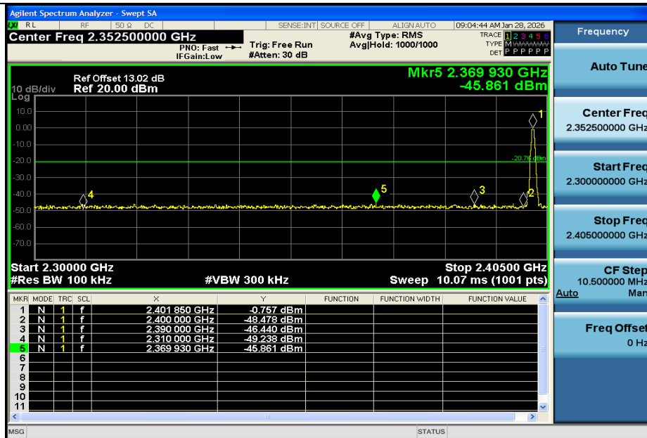
DH5-Ant1-2402-PASS
