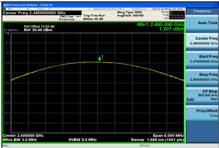
2DH5-Ant1-2480-PASS
