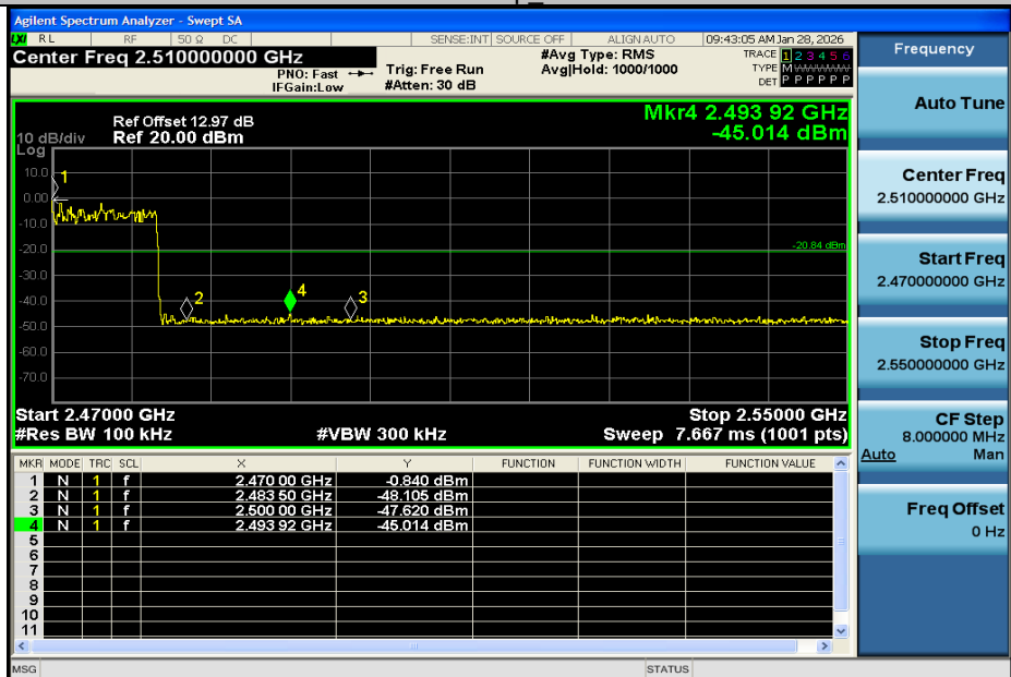
3DH5-Ant1-Hop_2480-PASS
