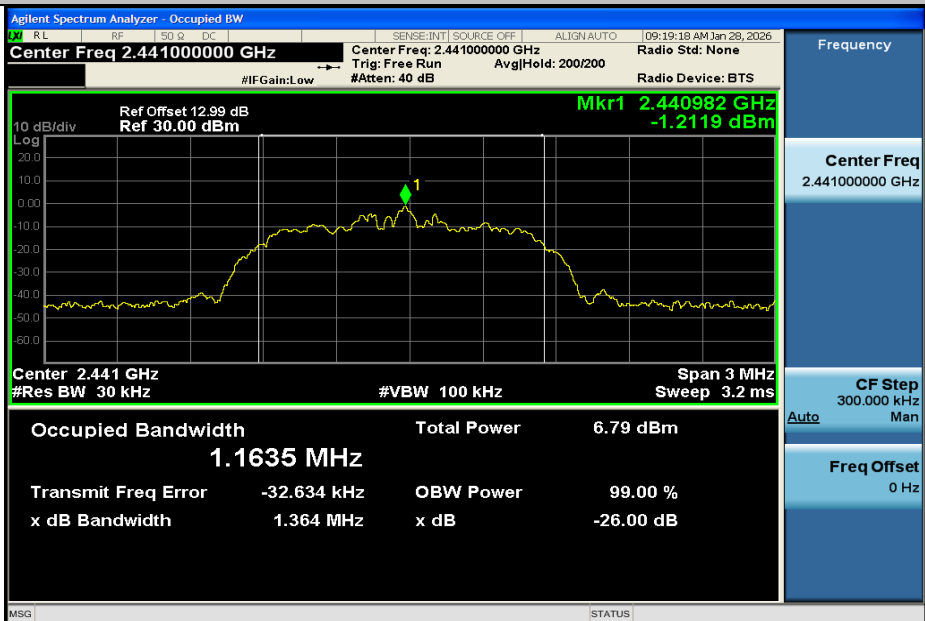
2DH5-Ant1-2441
