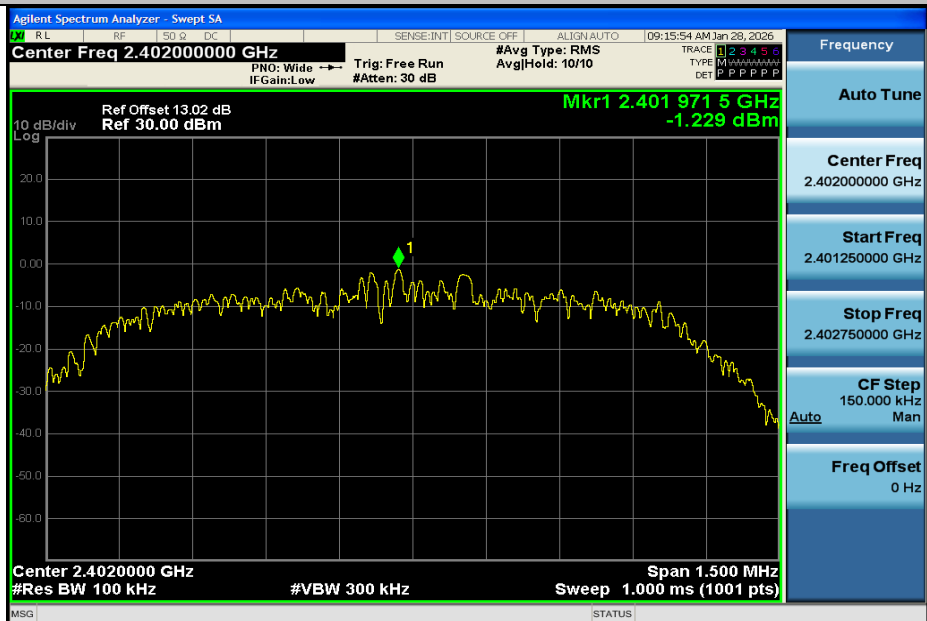
2DH5-Ant1-2402-0~Reference-PASS
