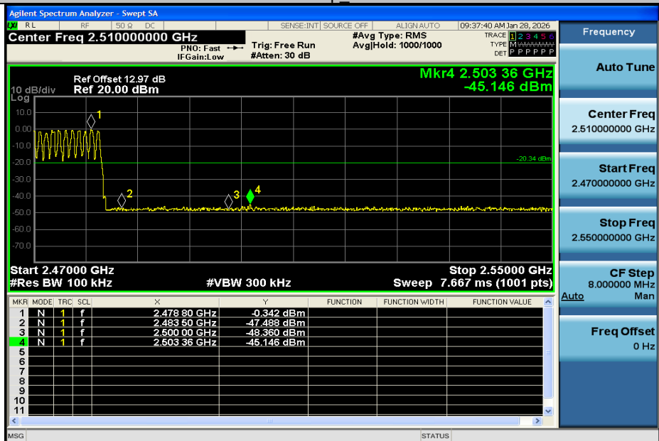
DH5-Ant1-Hop_2480-PASS
