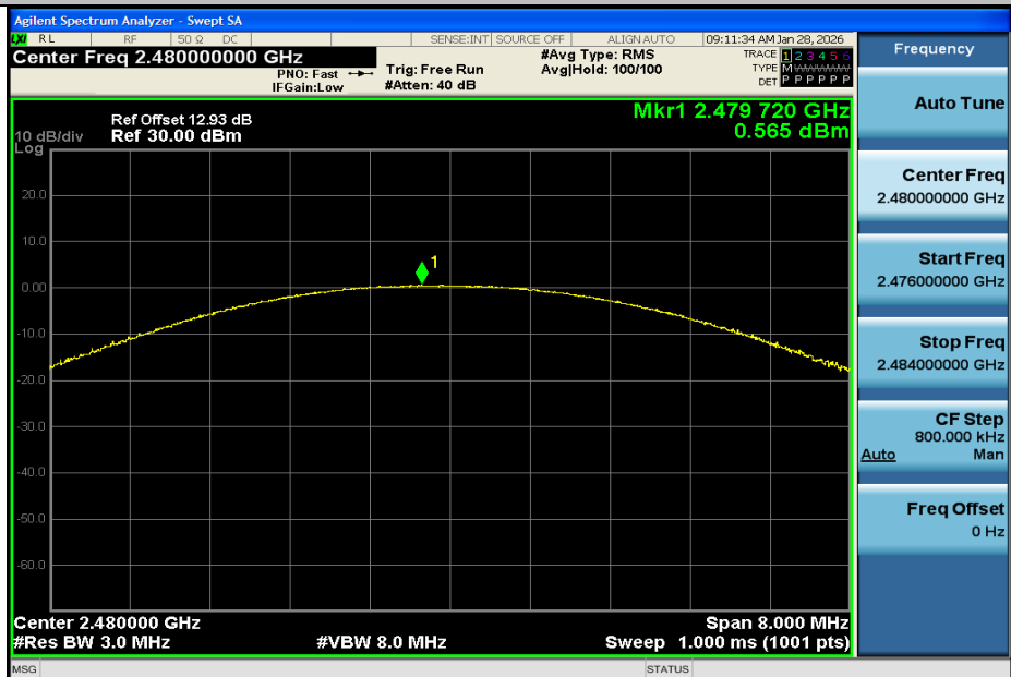
DH5-Ant1-2480-PASS
