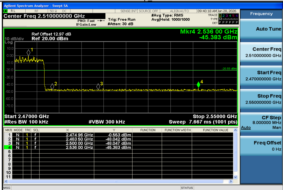
2DH5-Ant1-Hop_2480-PASS
