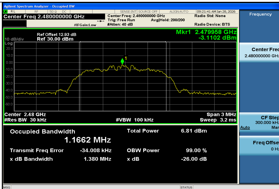
2DH5-Ant1-2480
