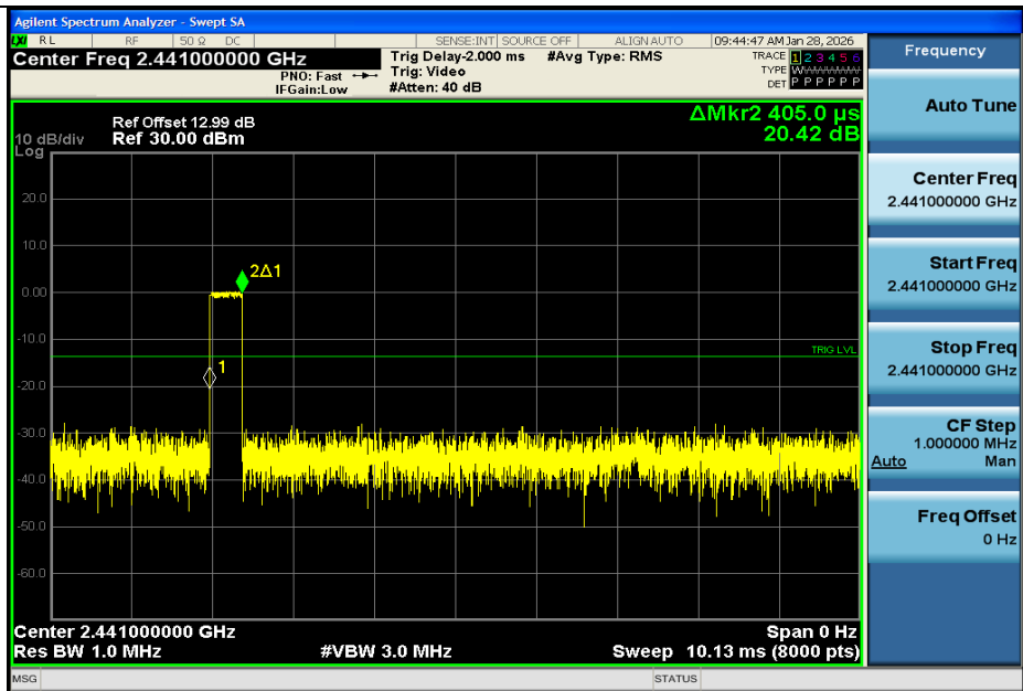
DH1-Ant1-Hop-PASS
