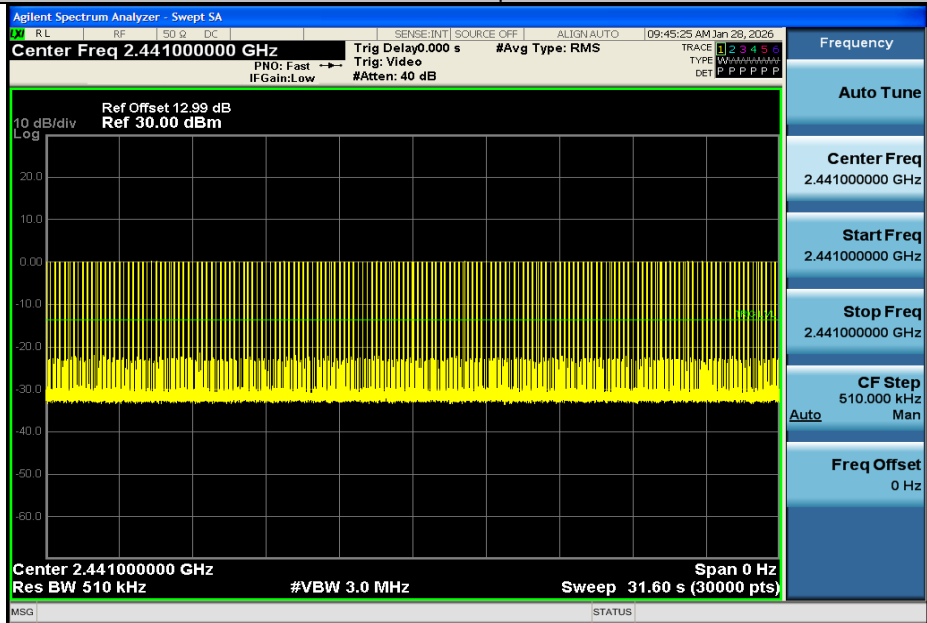
DH1-Ant1-Hop-PASS
