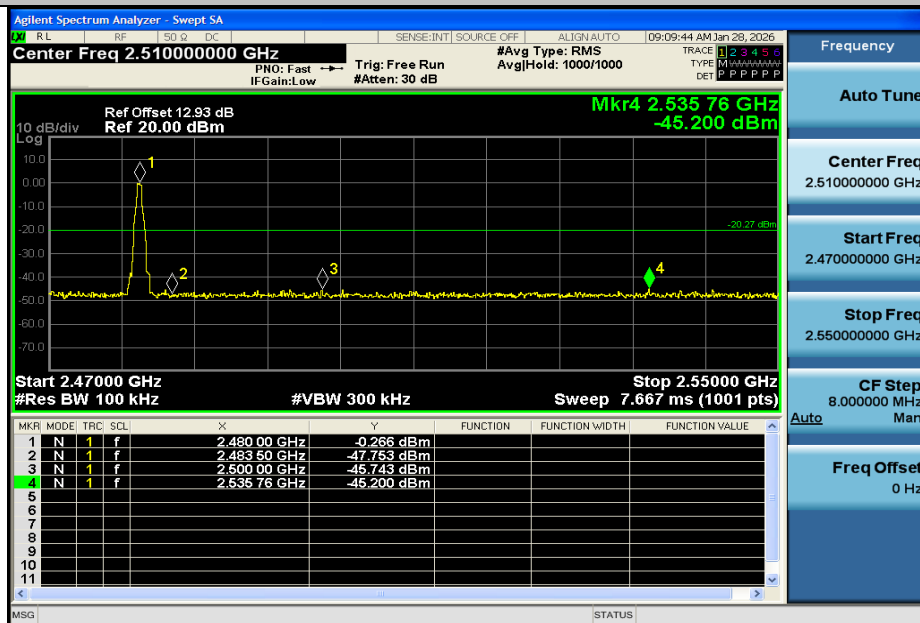
DH5-Ant1-2480-PASS
