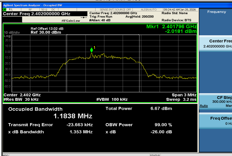
3DH5-Ant1-2402
