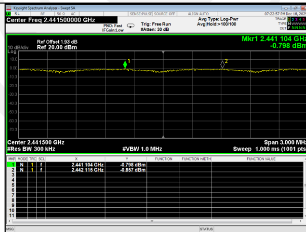
Carrier_Frequencies_Separation_(Hopping)_NVNT_ANT1_2-DH1_Hopping
