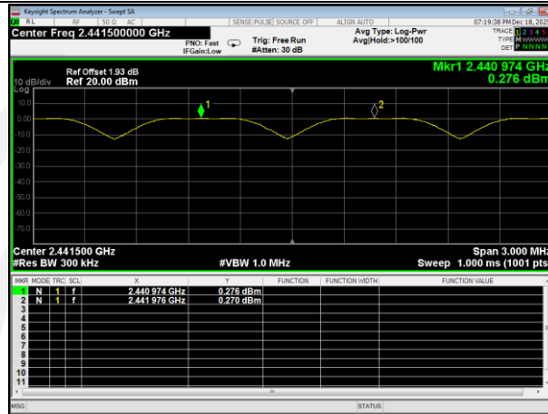
Carrier_Frequencies_Separation_(Hopping)_NVNT_ANT1_1-DH1_Hopping
