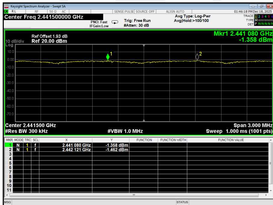
Carrier_Frequencies_Separation_(Hopping)_NVNT_ANT1_2-DH1_Hopping
