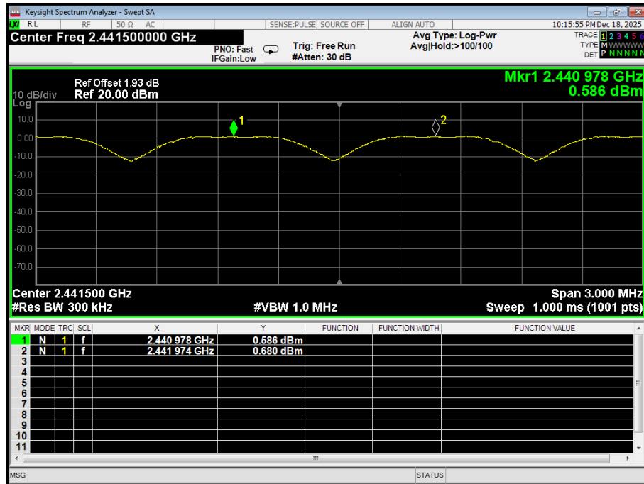
Carrier_Frequencies_Separation_(Hopping)_NVNT_ANT1_1-DH1_Hopping
