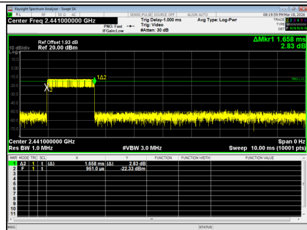
1DH5-2441MHz-One burst
