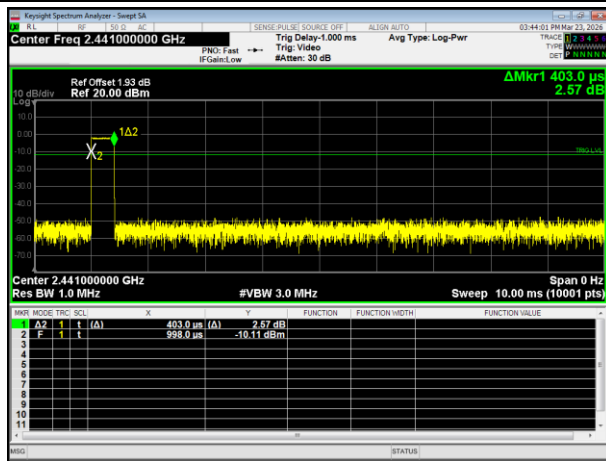
1DH3-2441MHz-One burst
