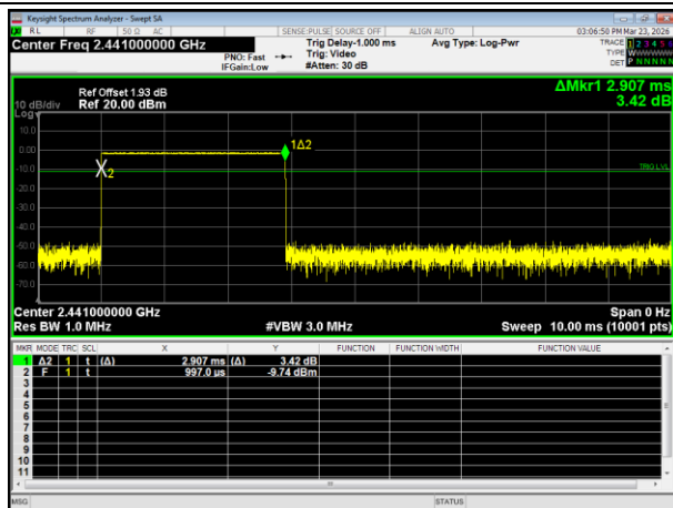
1DH5-2441MHz-One burst
