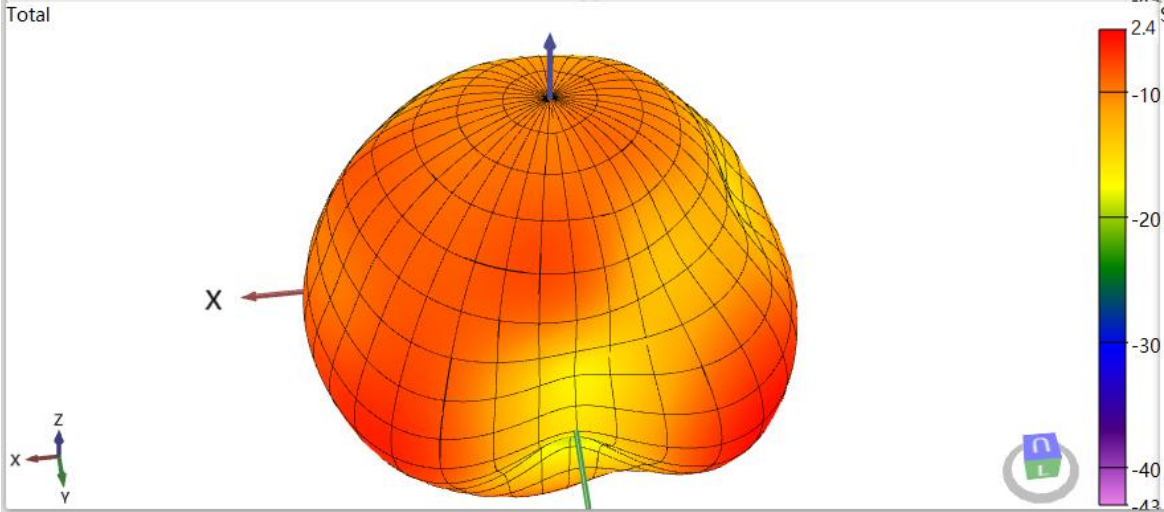
2500MHz 3D-Total Pattern
