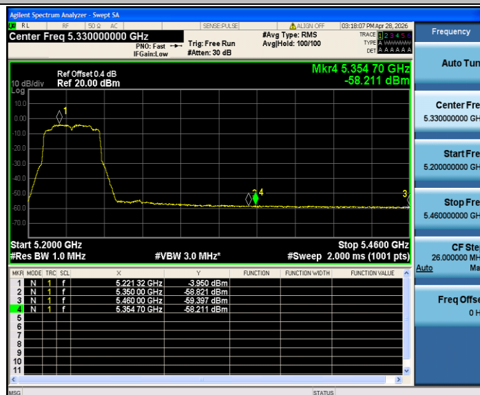
11AX40SISO_Ant2_High_5230_AV
