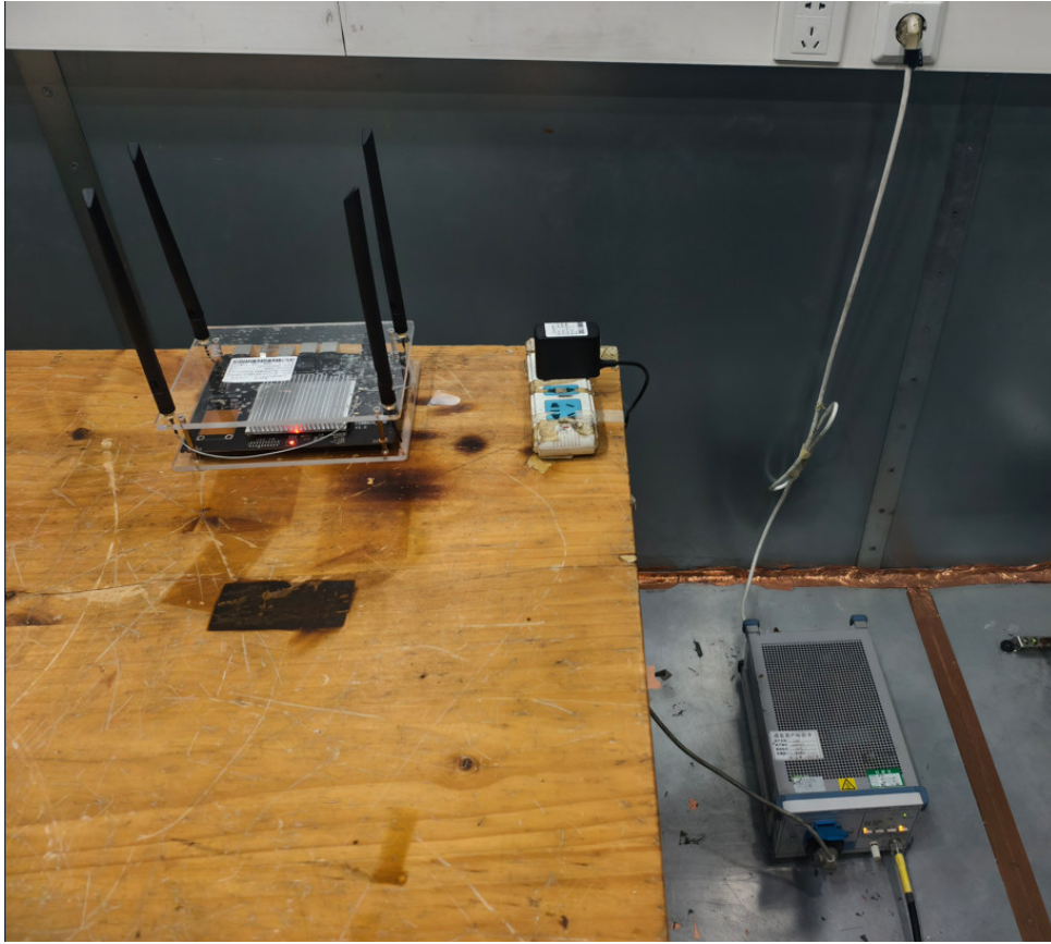
Picture 2: Conducted Emissions Test Setup
