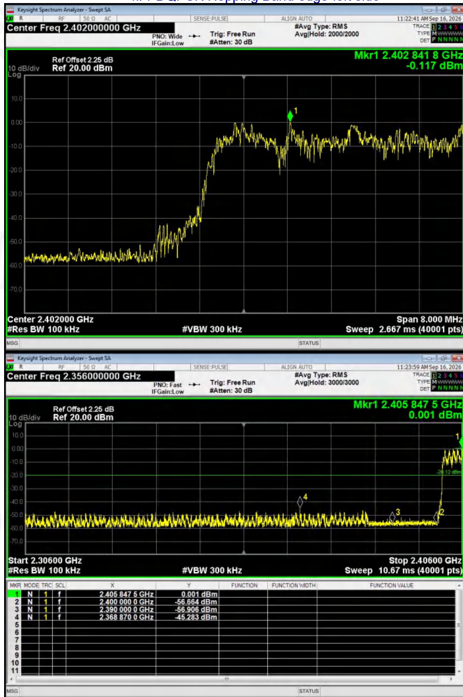
\pi/4 -DQPSK Hopping Band edge-left side
