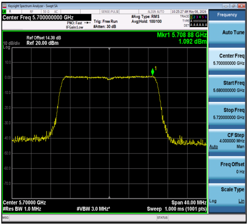
11AX20SISO-Ant1-5700-PASS
