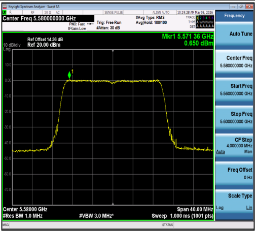
11AX20SISO-Ant1-5580-PASS
