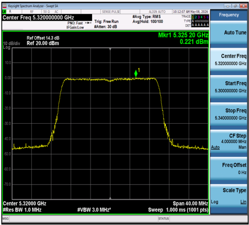
11AX20SISO-Ant1-5320-PASS
