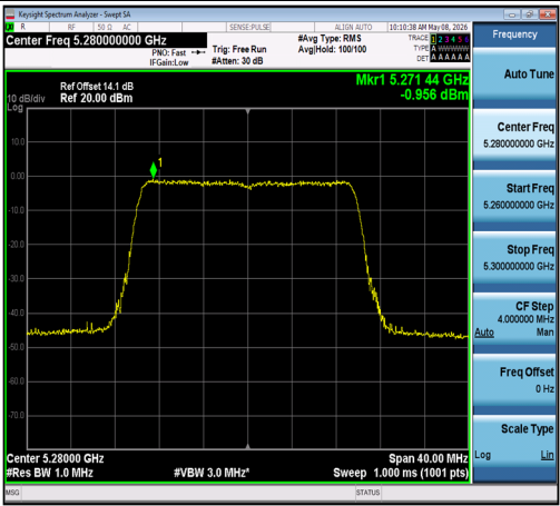
11AX20SISO-Ant1-5280-PASS
