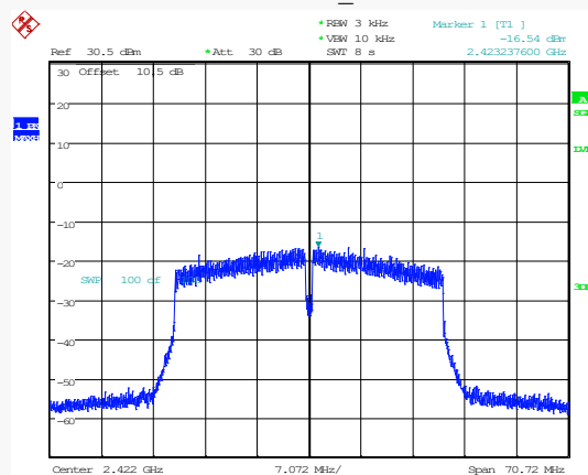
802.11n40_2422MHz
