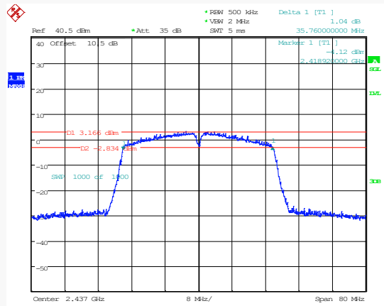
802.11n40_2437MHz
