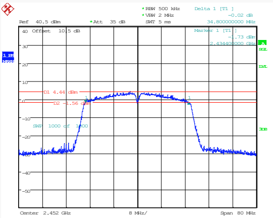
802.11n40_2452MHz
