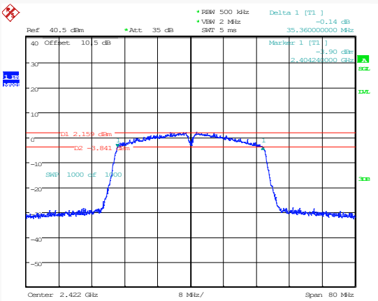
802.11n40_2422MHz
