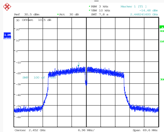
802.11n40_2452MHz
