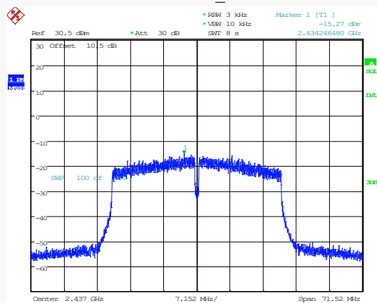
802.11n40_2437MHz
