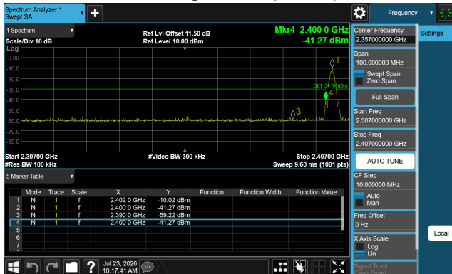
Bandedge CH00 (Lower)
