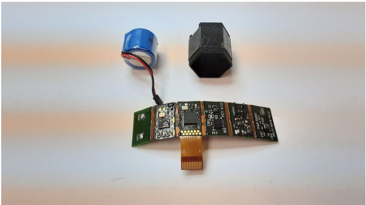
Hex Carrier Assembly Removed
