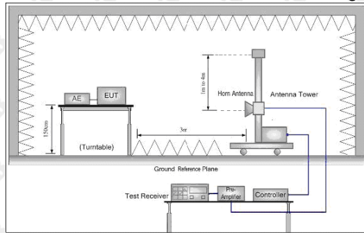
Figure 3. Above 1GHz
