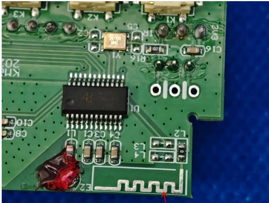
PCB Antenna
