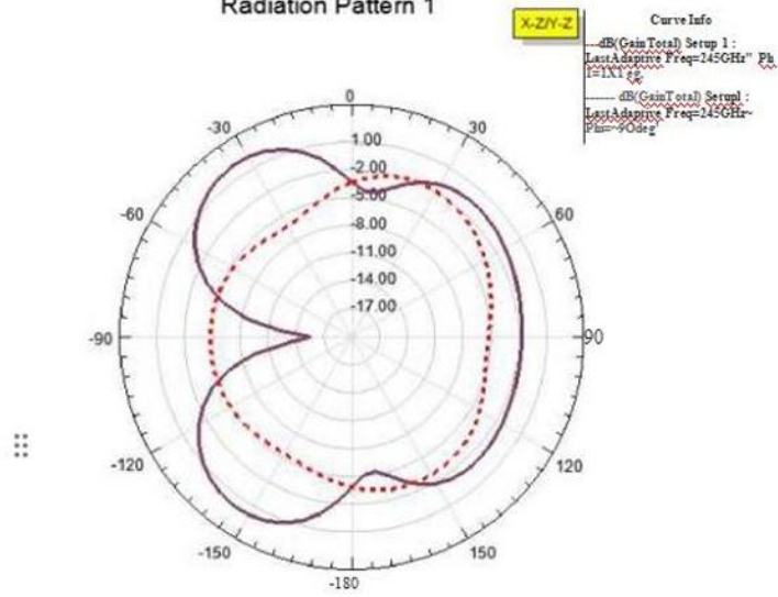
Radiation Pattern 1
