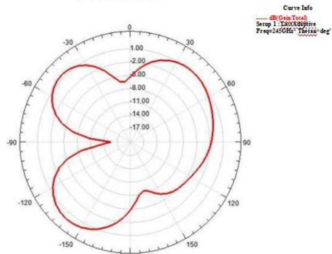
Radiation Pattern 2
