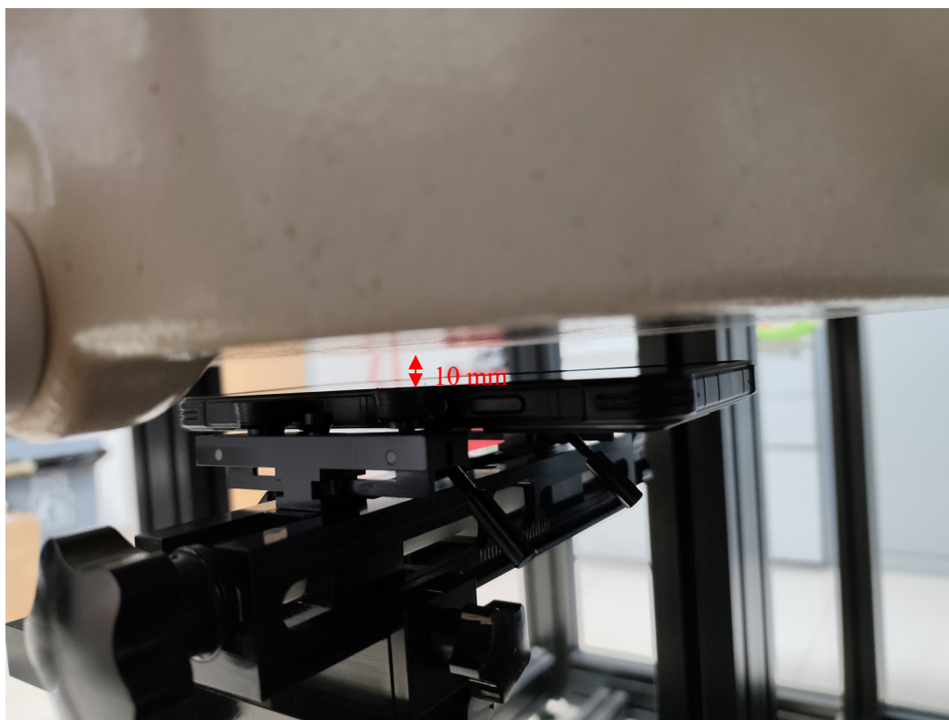
ANT4 Body Back Setup Photo (10 mm)
