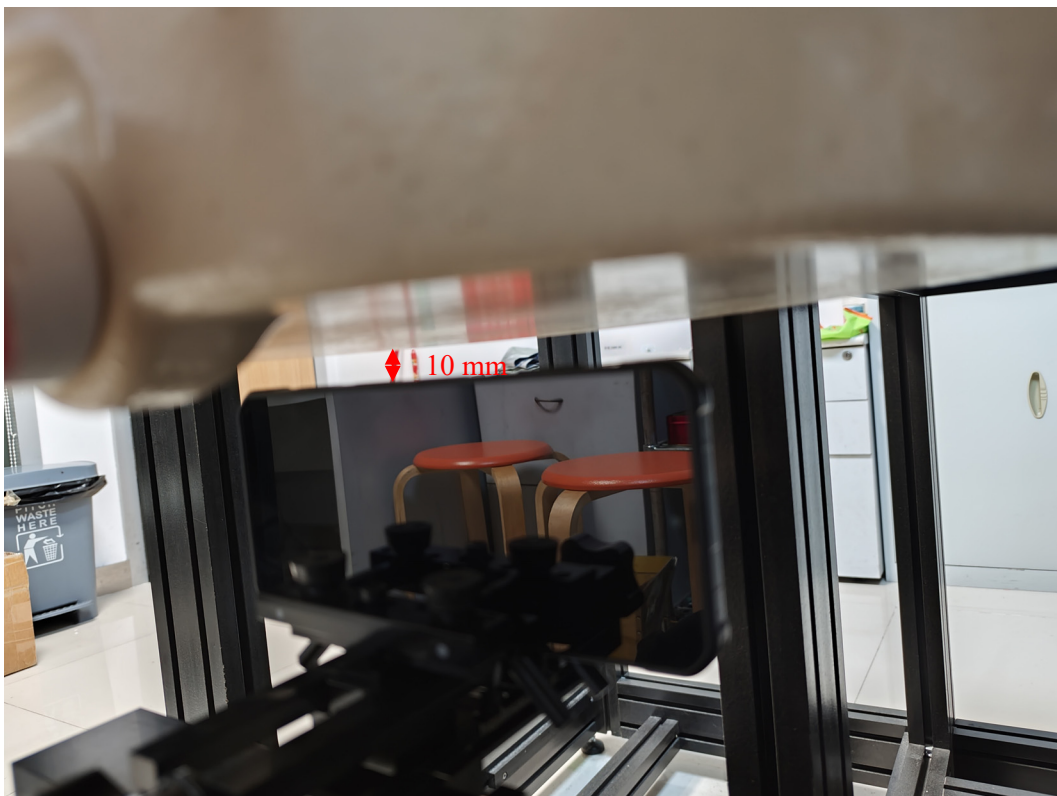
ANT4 Body Left Setup Photo (10 mm)
